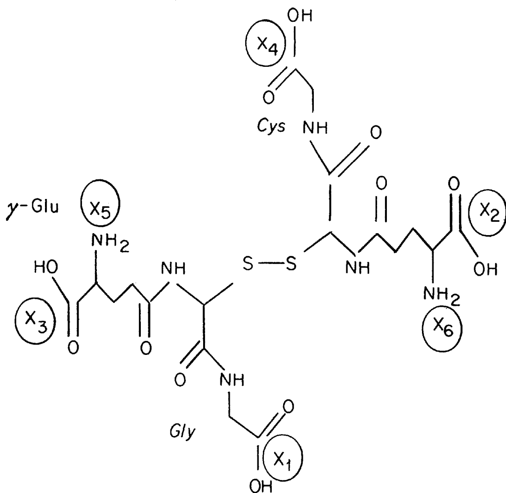
Glutathione oxidized
