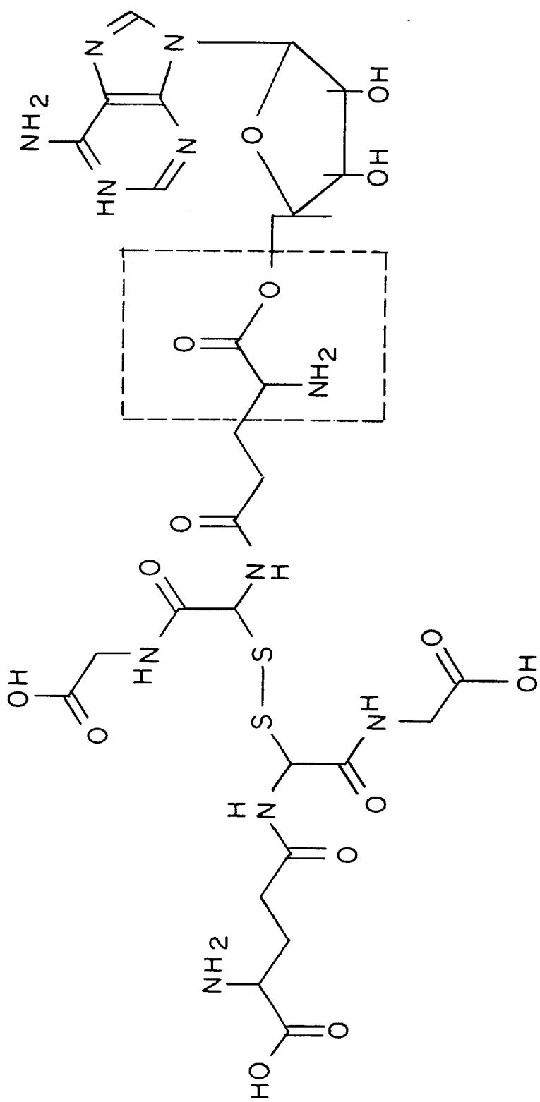
[9-β-D-ribofuranosyladenyl]·glutathione disulfide
