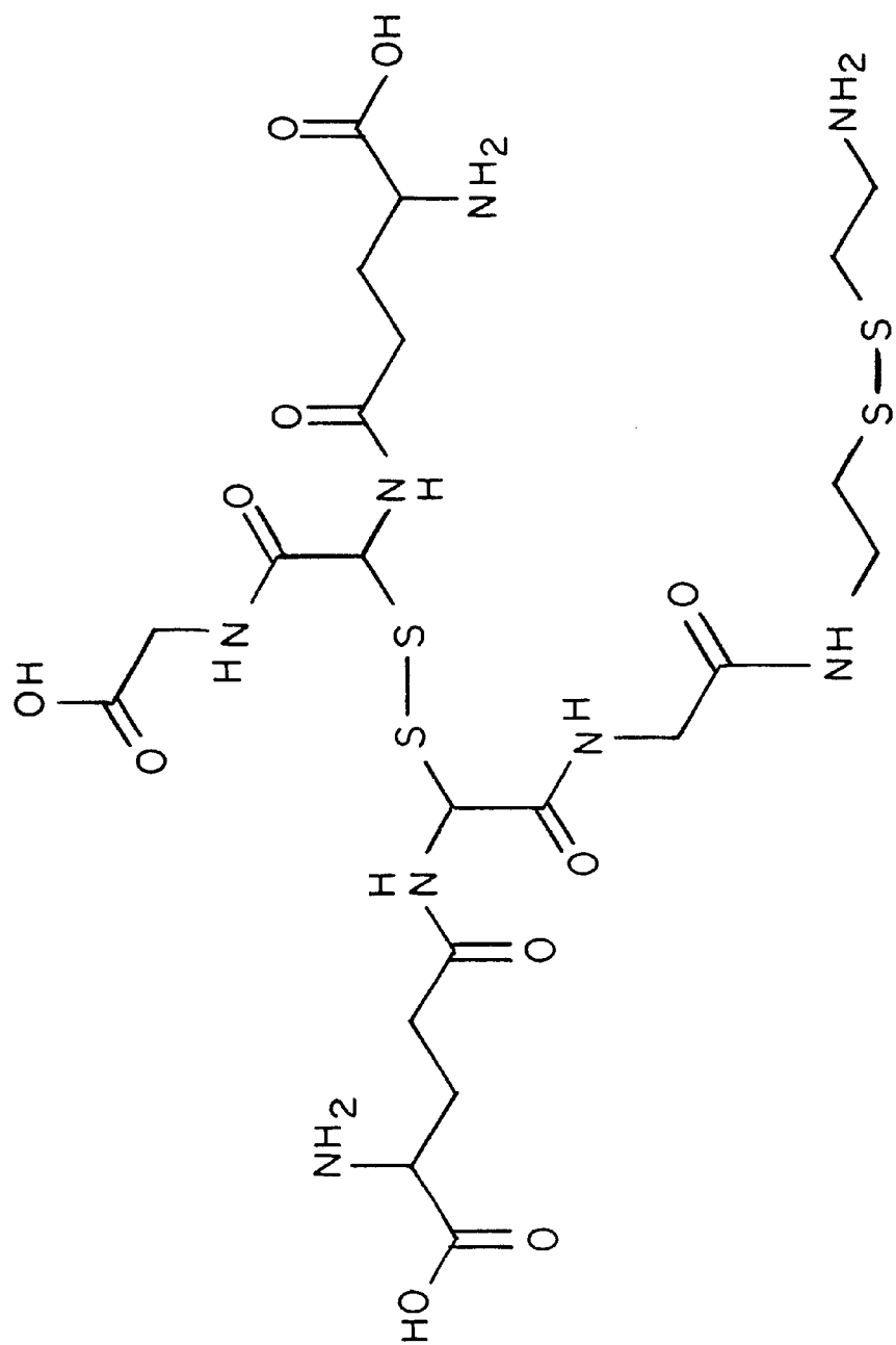
S-thioethylamine-glutathione disulfide
