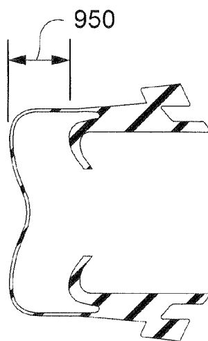
Fig. 95C SECTION B-B
