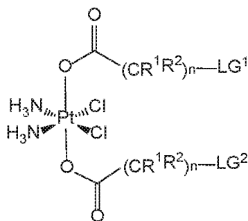
Formula IB
