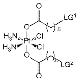
Formula IA
