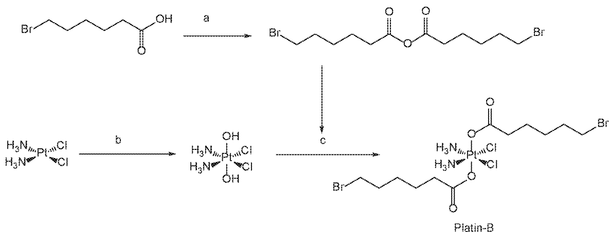
Scheme 1. Synthesis of Platin-B from cisplatin and 6-BH. A) DCC, CH 2 Cl 2 , 25 °C, 12 h, quantitative yield; b) H 2 O 2 , 75 °C, 5h, 90 %; c) DMF, 25 °C, 12 h, 64 %.
