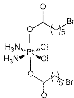
Formula IA-1 (Platin-B)
