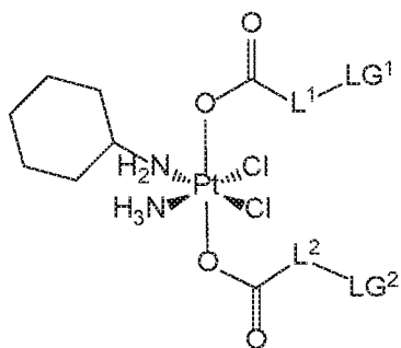
Formula IV
