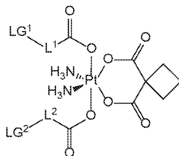
Formula II
