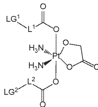
Formula VI
