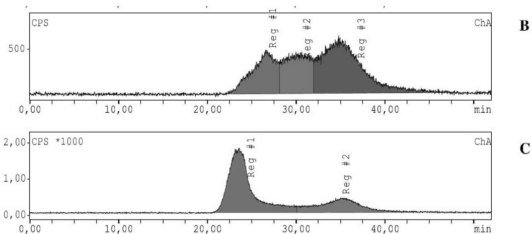
Figure 2: Size exclusion radio-chromatograms of (A) ^{177}\text{Lu} -CC49-TCO and ^{177}\text{Lu} -CC49-TCO in the presence of bovine submaxillary mucin type I-S (BSM) (B) before and (C) after 1 hr reaction with tetrazine 7
