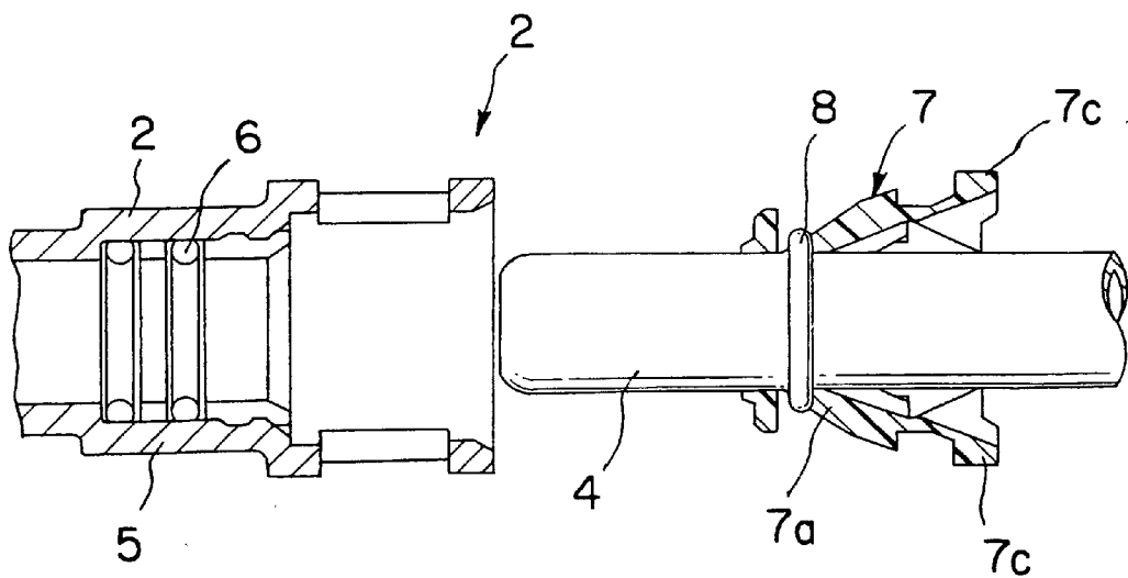
FIG. 21 (Prior Art)
