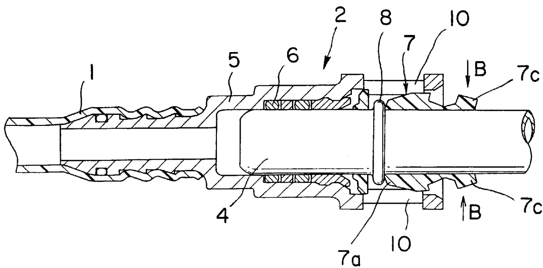
FIG. 20 (Prior Art)
