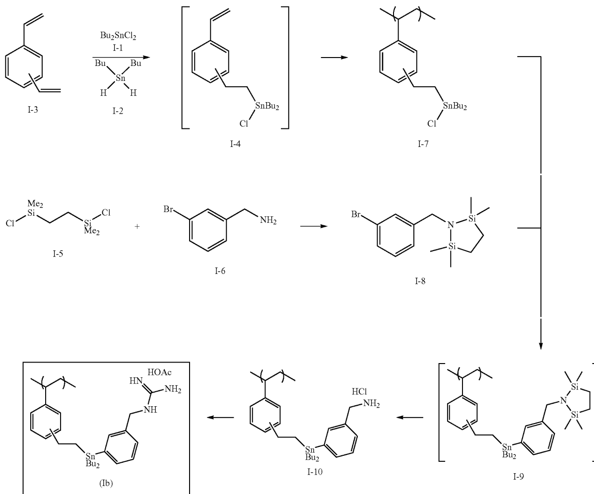
Scheme 2: Synthetic Route to Polymer Comprising Monomer of Formula (I)
