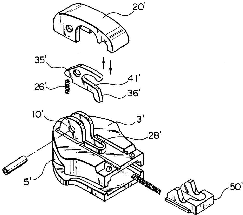
FIG. 10 PRIOR ART
