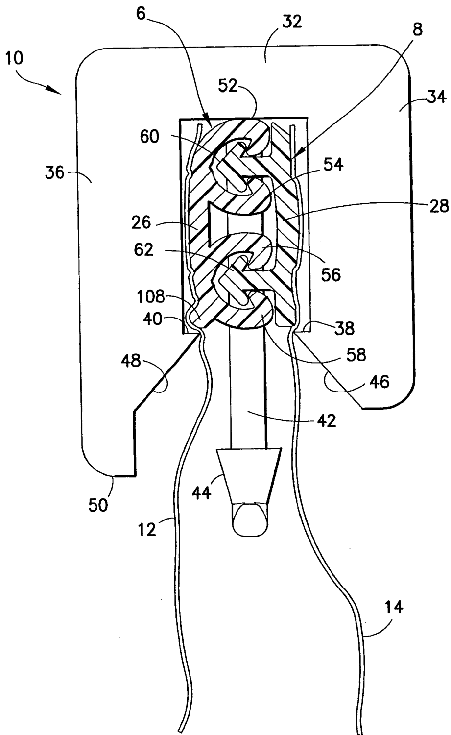
FIG. 2 PRIOR ART
