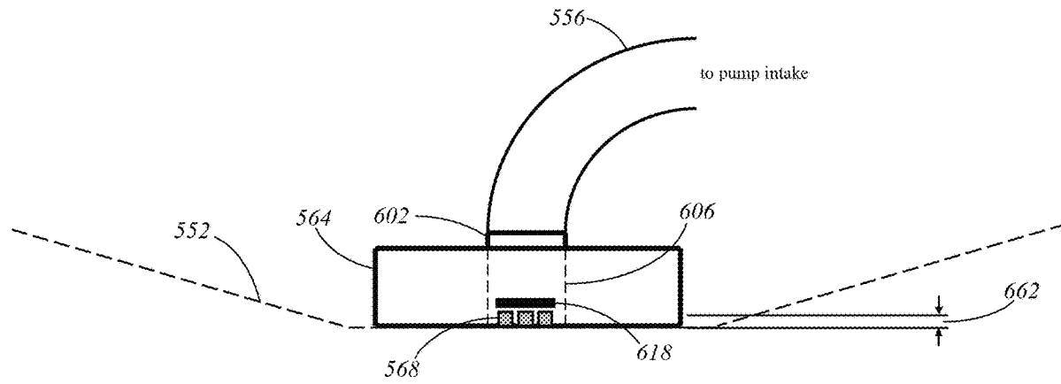
Figure 11 side view
