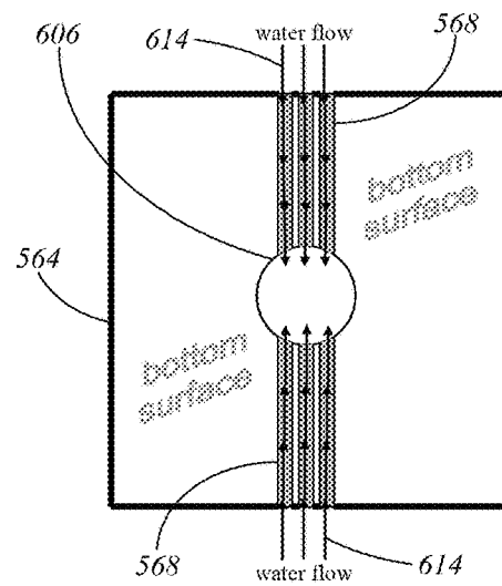
Figure 12 bottom view
