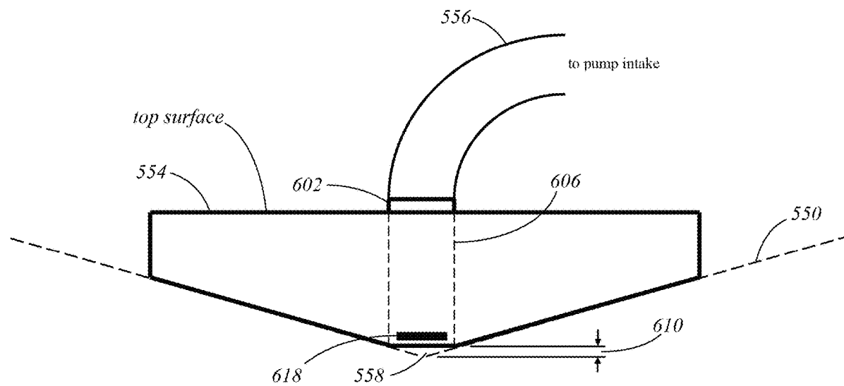
Figure 9 side view
