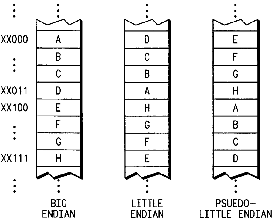
2 x 4-BYTE TRANSFERS
