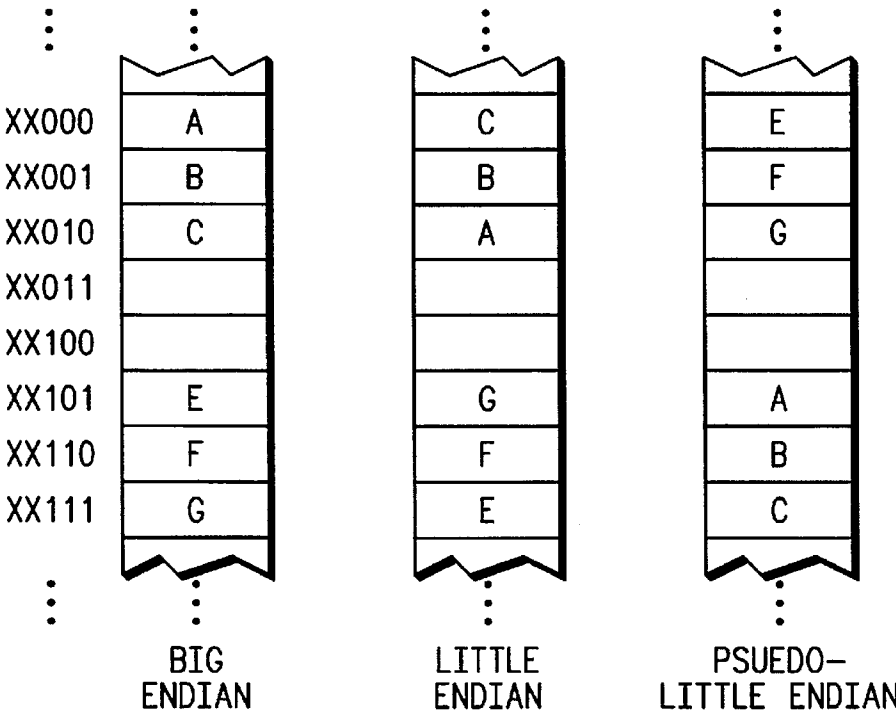
2 x 3-BYTE TRANSFERS
