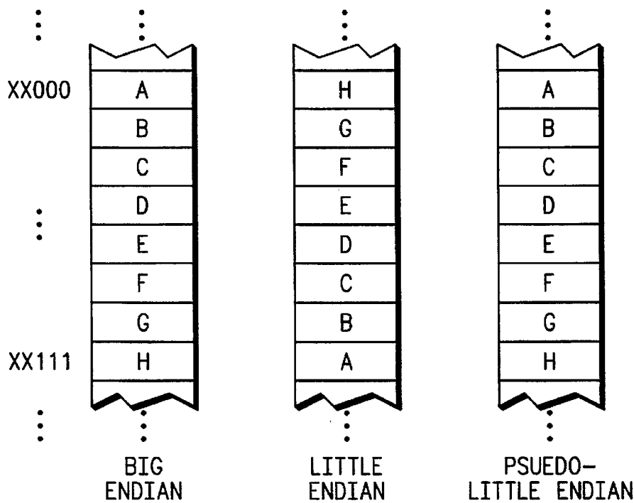
1 x 8-BYTE TRANSFER FIG.2
