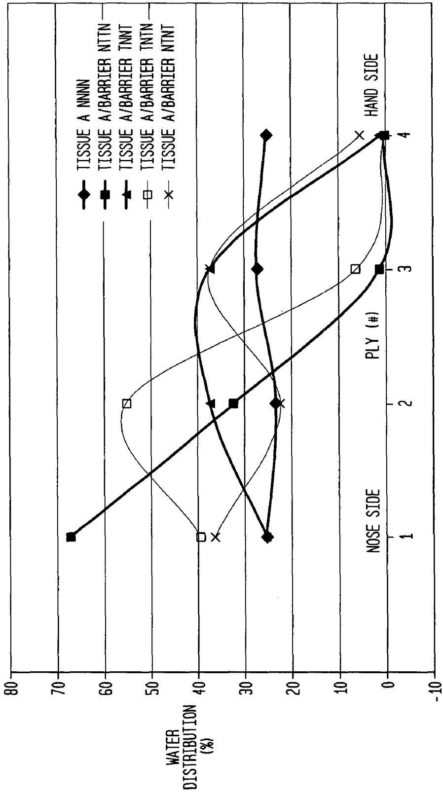
FIG. 31 4-PLY STERNUTATION TESTING
