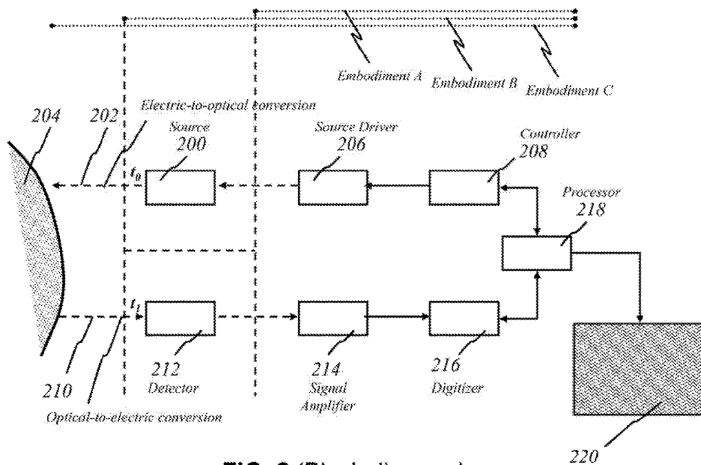
FIG. 2 (Block diagram)
