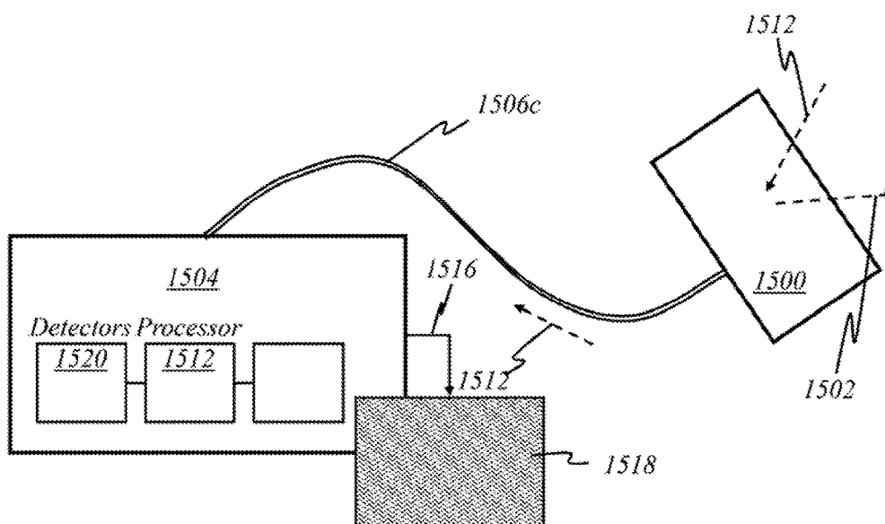
FIG. 17 Whole view (with optical fiber) (1)
