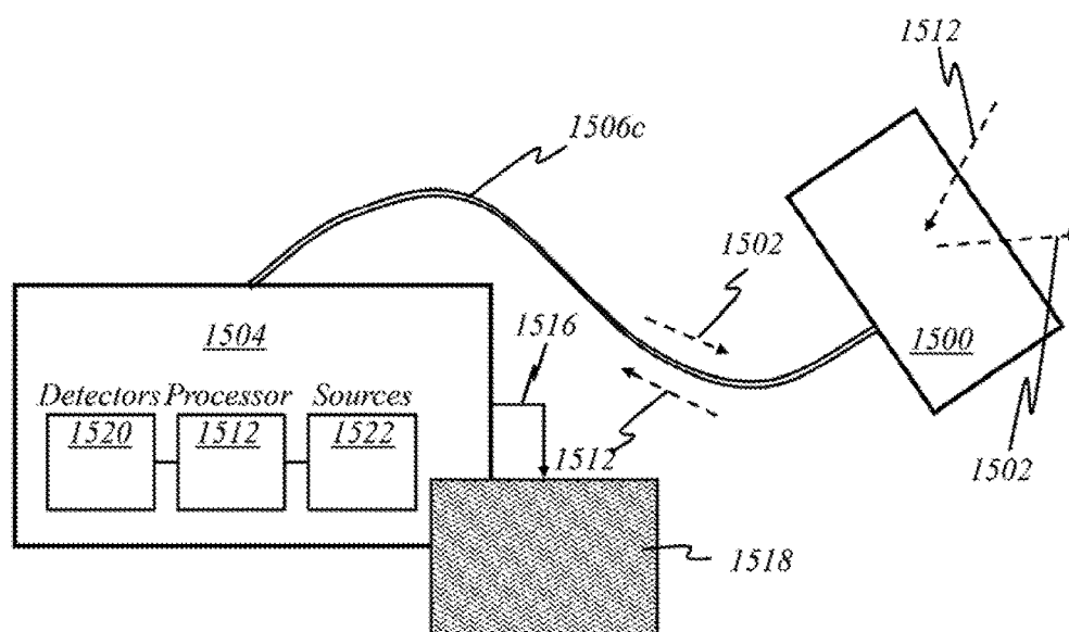
FIG. 18 Whole view (with optical fiber) (2)
