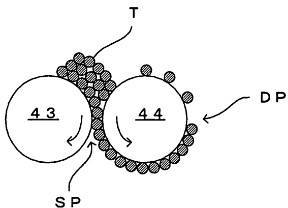
FIG. 4A : GREAT RESIDUAL QUANTITY OF TONER
