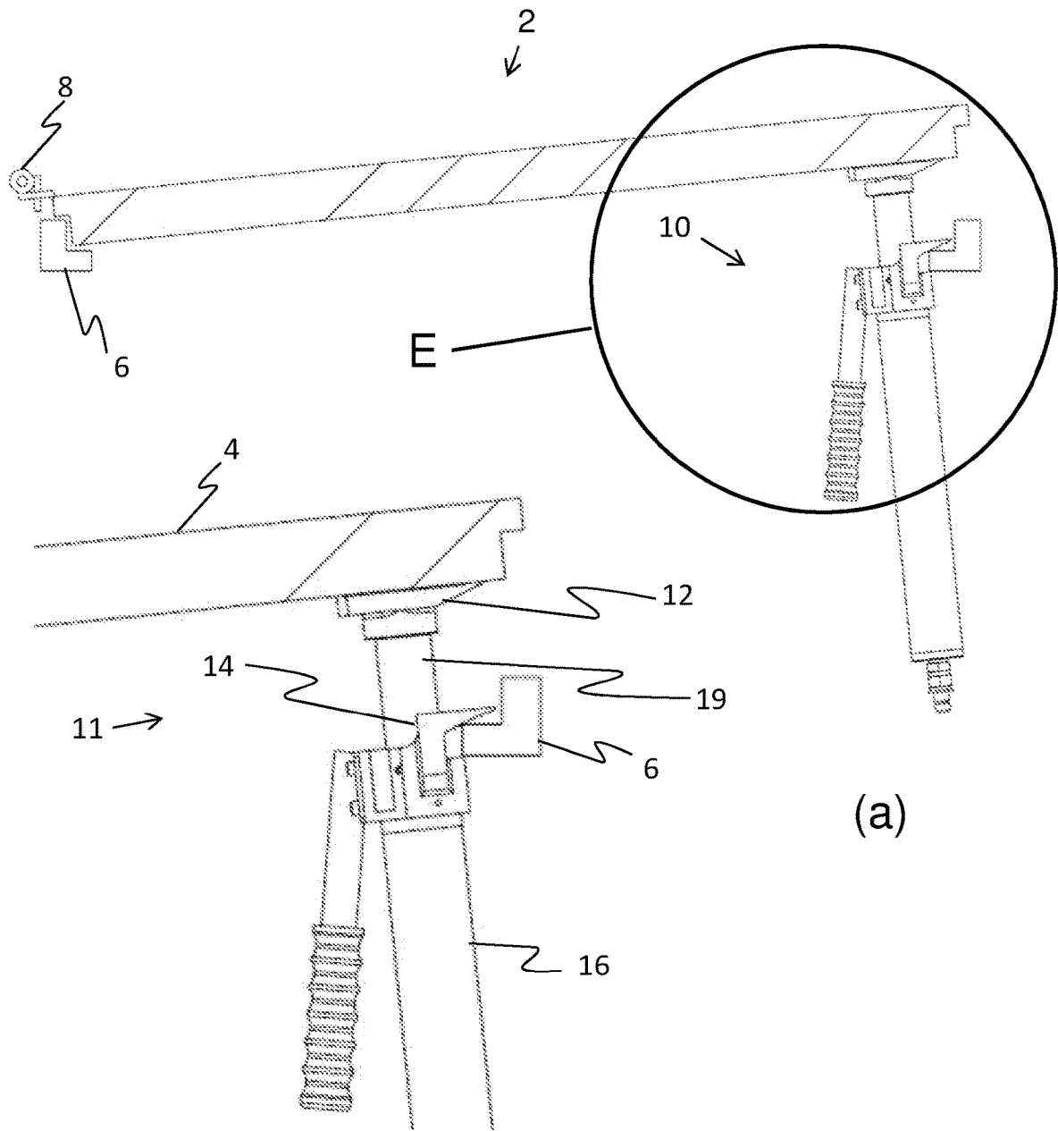
DETAIL "E"
