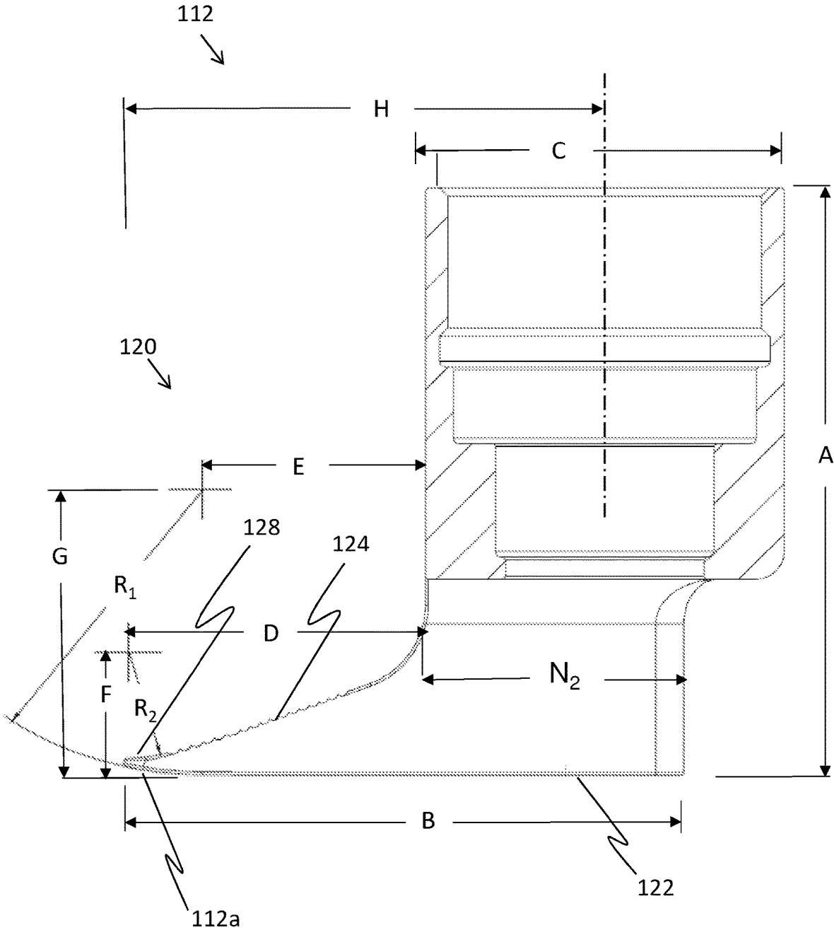
SECTION W-W
