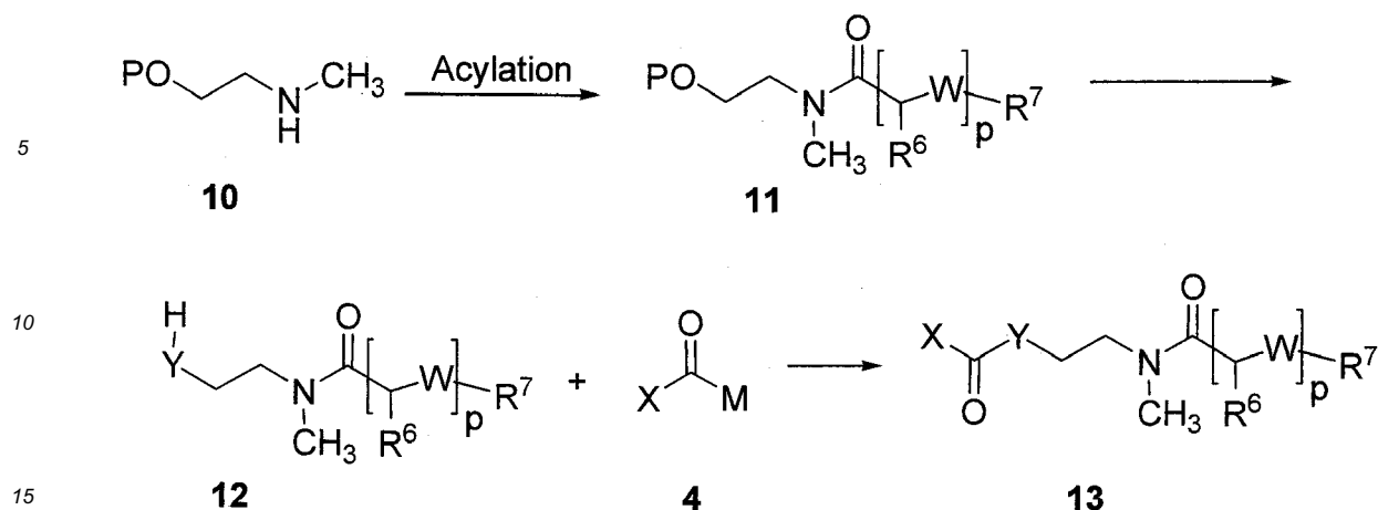
Scheme 3
