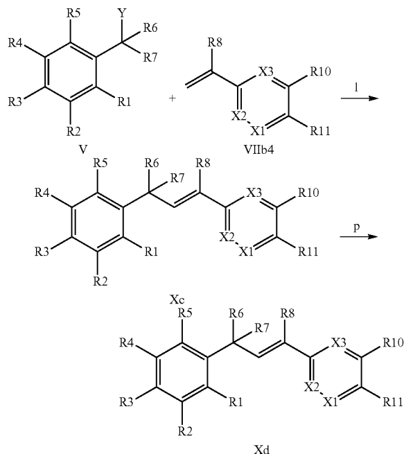
Scheme X
