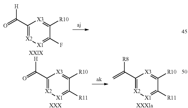
Scheme XXVII
