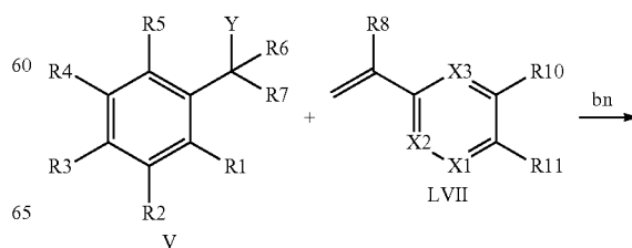
Scheme XL
