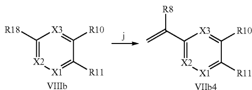
Scheme IX
