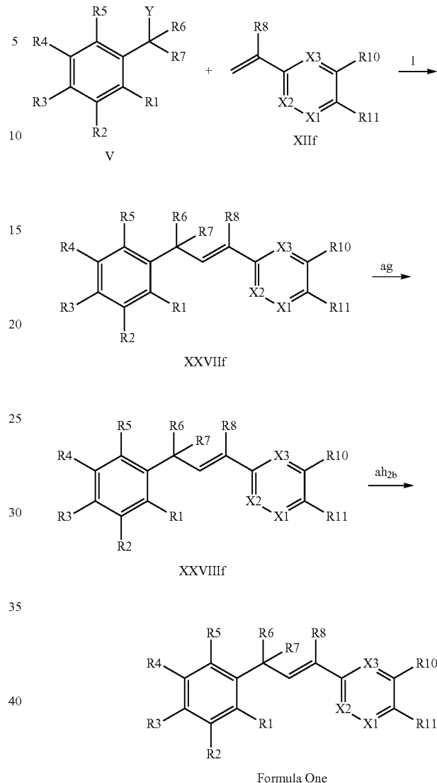
Scheme XXV
