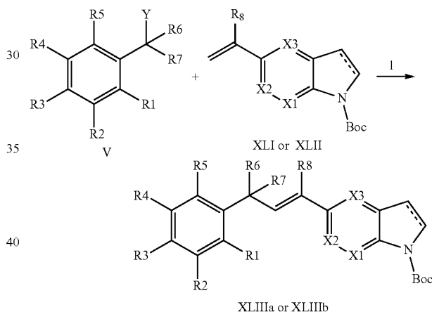
Scheme XXXV
