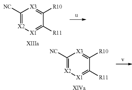
Scheme XIV
