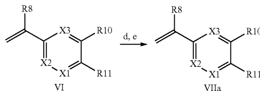
Scheme II
