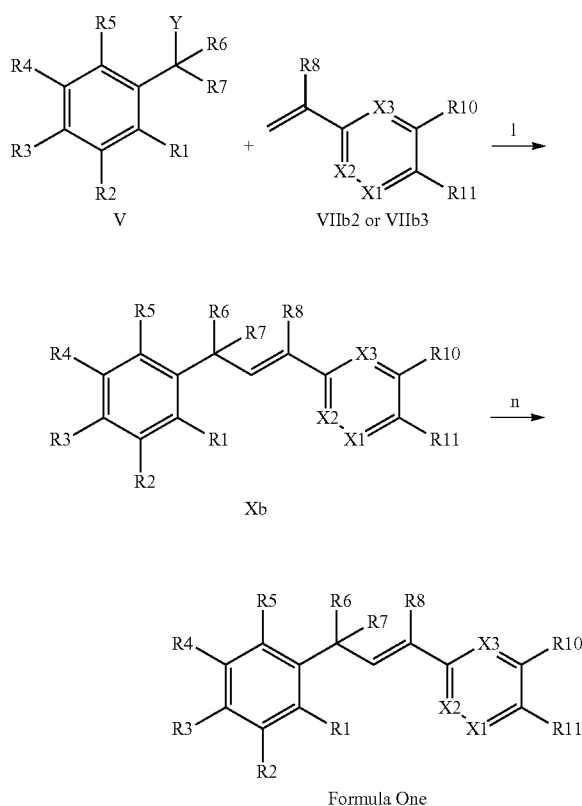
Scheme VIII
