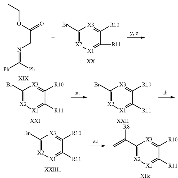
Scheme XVI
