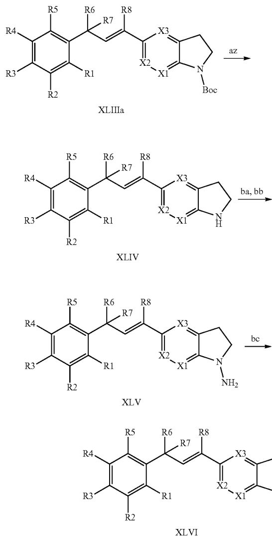
Scheme XXXVI
