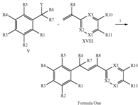
Scheme XXVI
