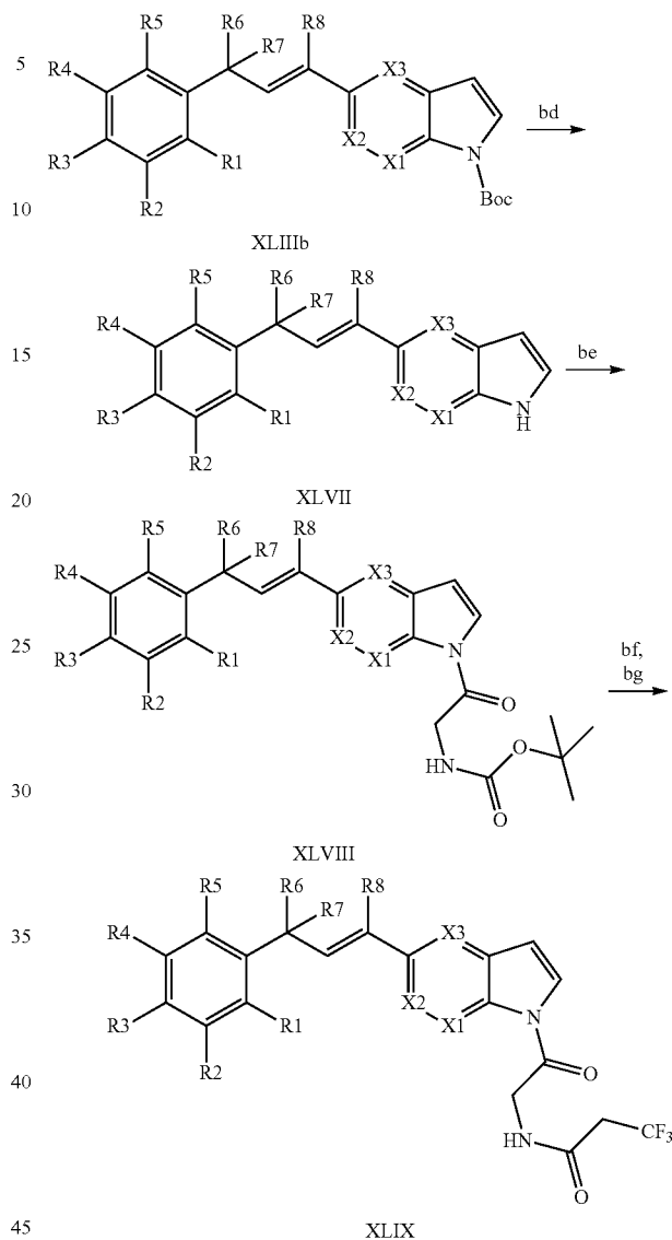
Scheme XXXVII
