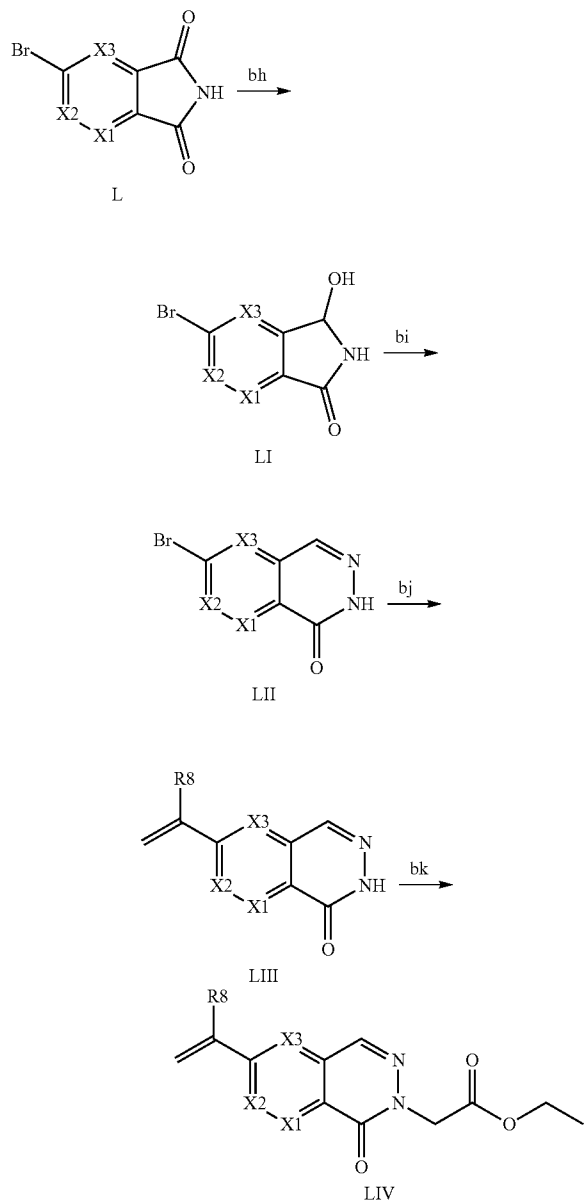
Scheme XXXVIII
