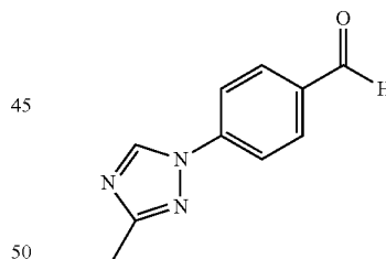
5-Methyl-4-(1H-1,2,4-triazol-1-yl)benzaldehyde (DI51)
