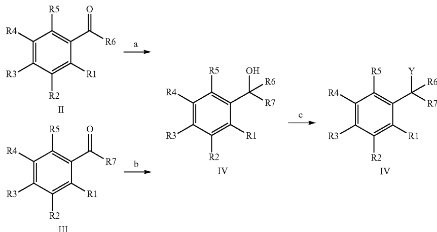
Scheme I
