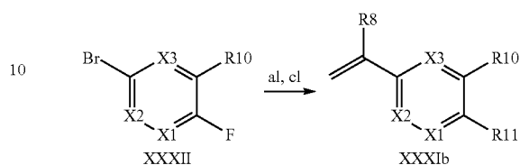
Scheme XXVIII
