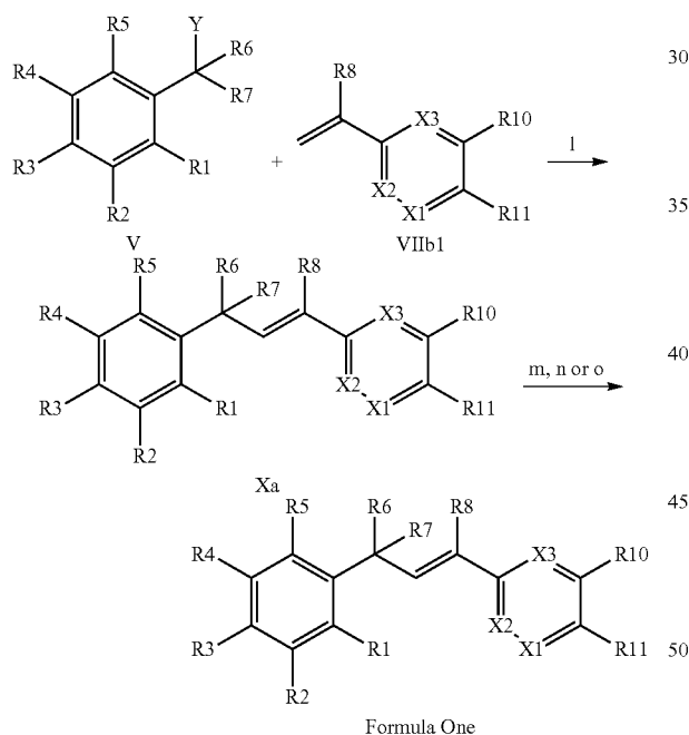
Scheme VII
