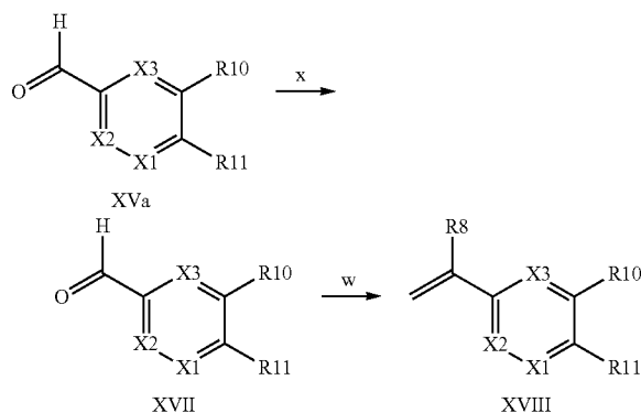
Scheme XV
