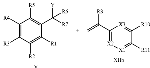
Scheme XXI
