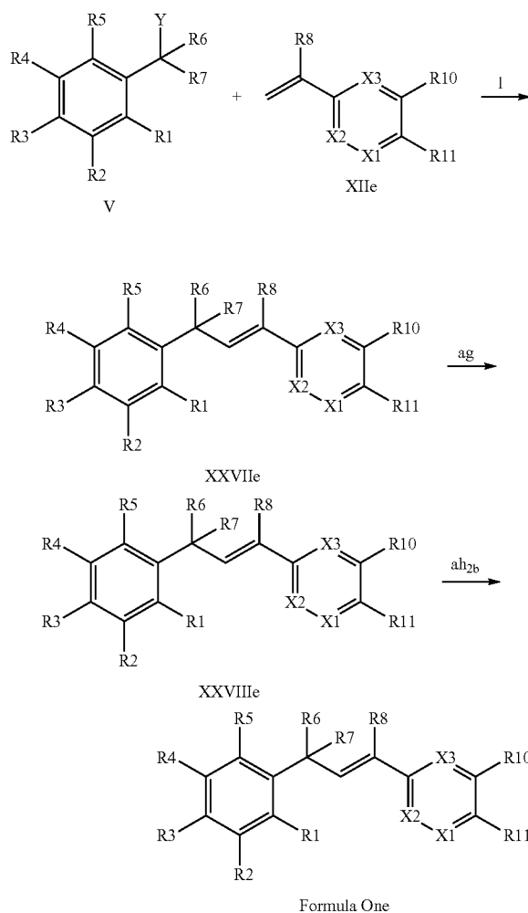
Scheme XXIV
