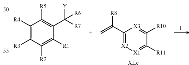
Scheme XXII
