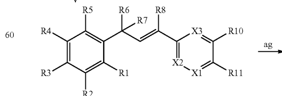
XXVIIIc
