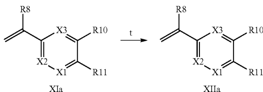
Scheme XIII
