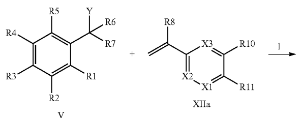
Scheme XX
