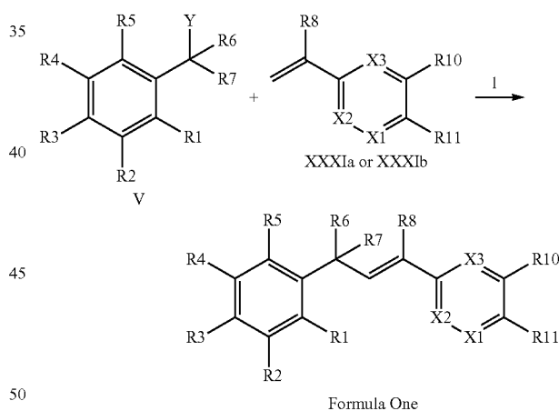
Scheme XXIX
