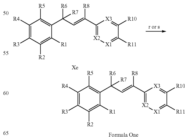
Scheme XII
