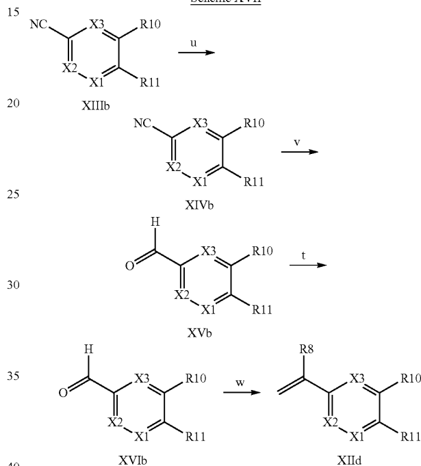
Scheme XVII
