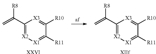
Scheme XIX
