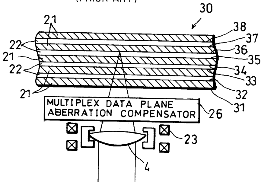
FIG. 18 (PRIOR ART)
