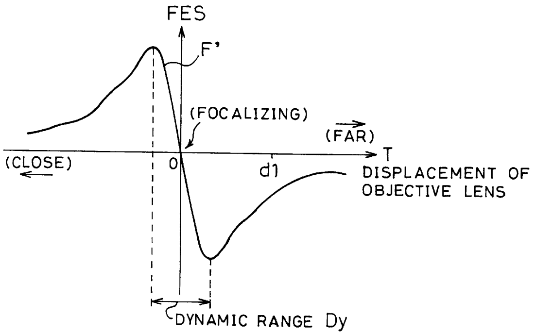
FIG. 23 (PRIOR ART)
