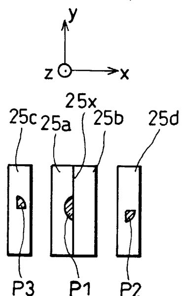
FIG. 22(c) (PRIOR ART)
