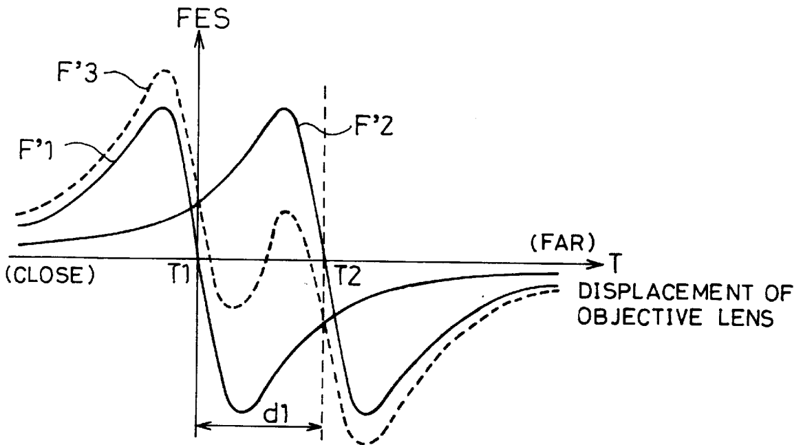
FIG. 24 (PRIOR ART)
