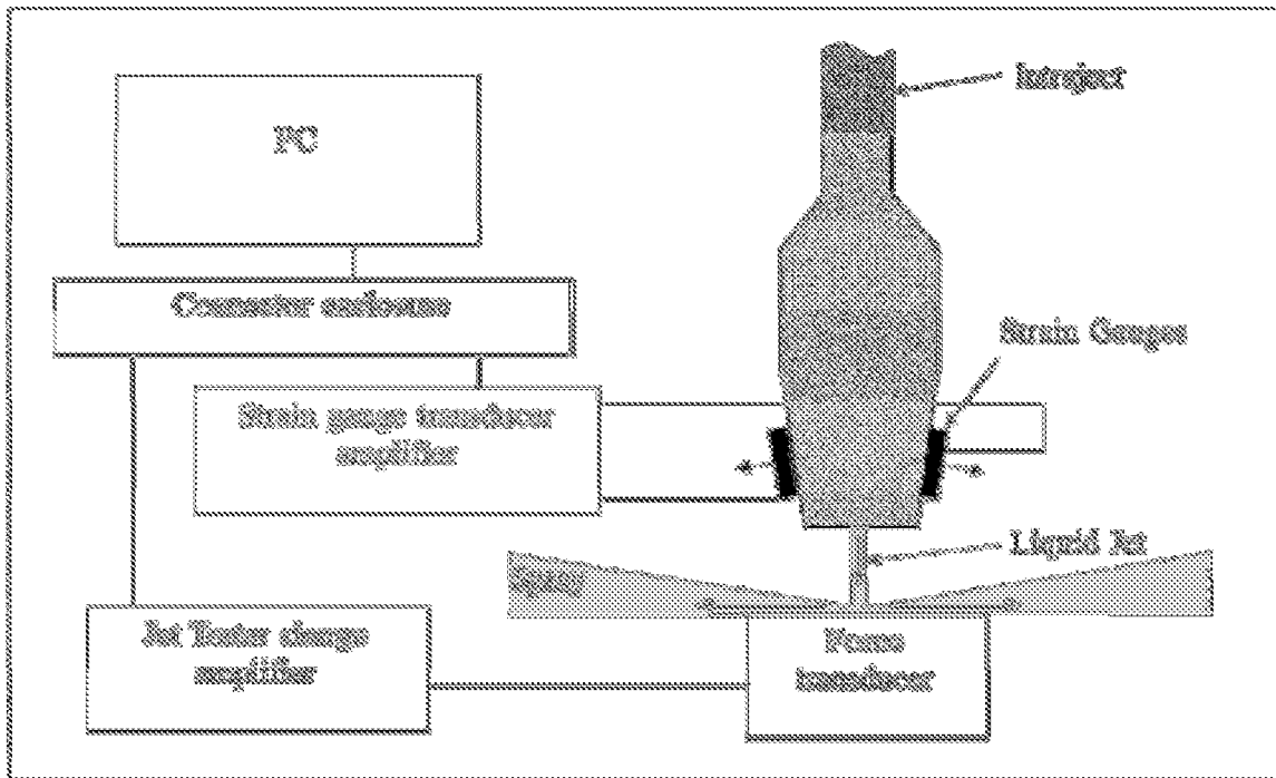
Figure 4: Schematic of Jet Tester Used to Measure Formulation Pressure vs. Time
