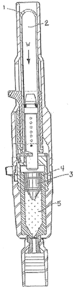
Figure 1: DosePro, a Needle Free Injector of a Preferred Embodiment of the Invention
