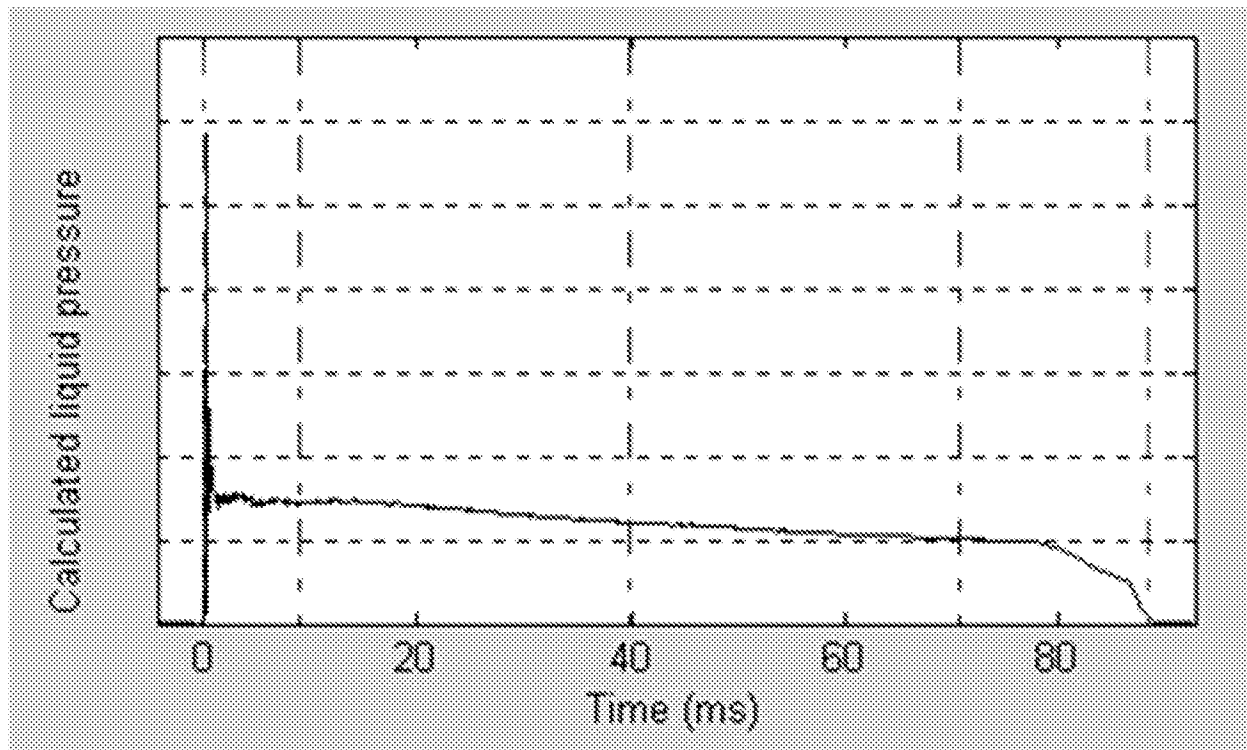
Figure 2: Drug Formulation Pressure vs. Time, Utilizing a 500 \mu L version of DosePro Showing the Initial Pressure Spike (“Puncture Phase”) and the Lower Pressure “Delivery Phase”
