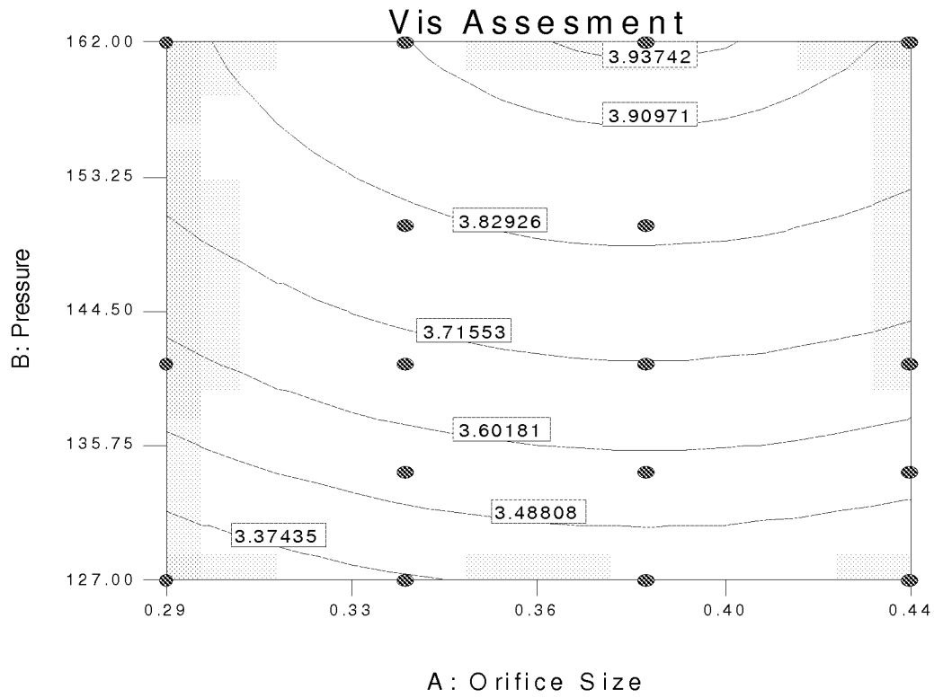
Figure 8: Gas Mass and Orifice Size Model Parameter Space and Prediction
