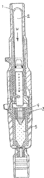
Figure 1: DosePro, a Needle Free Injector of a Preferred Embodiment of the Invention
