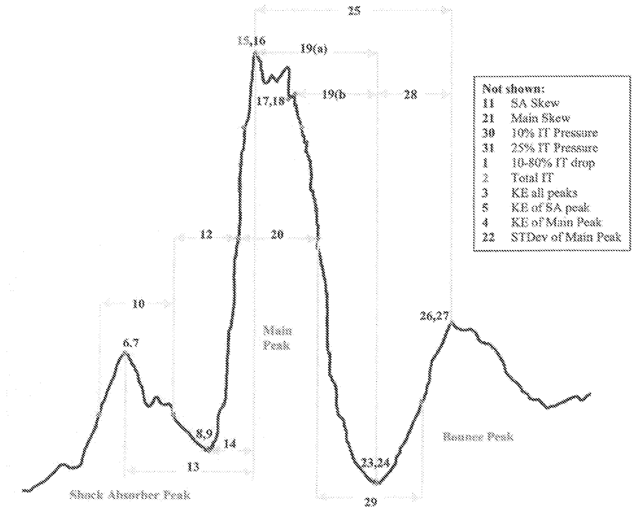
Figure 3: Capsule Pressure vs. Time, With Parameters that were Correlated with Quality of Injection
