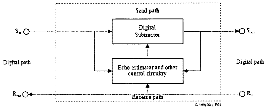
Digital transmission echo canceller using digital subtraction
