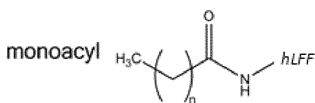
Figure 1: Structures of acylated and biacylated human lactoferrin peptides.
