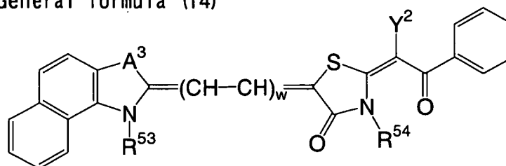
General formula (14)
