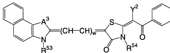
General formula (13)
