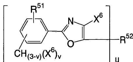
General formula (12)
