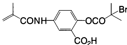
Monomer (A-1M)
