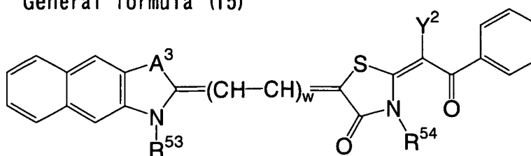
General formula (15)
