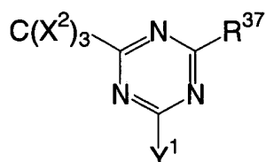
General formula (6)
