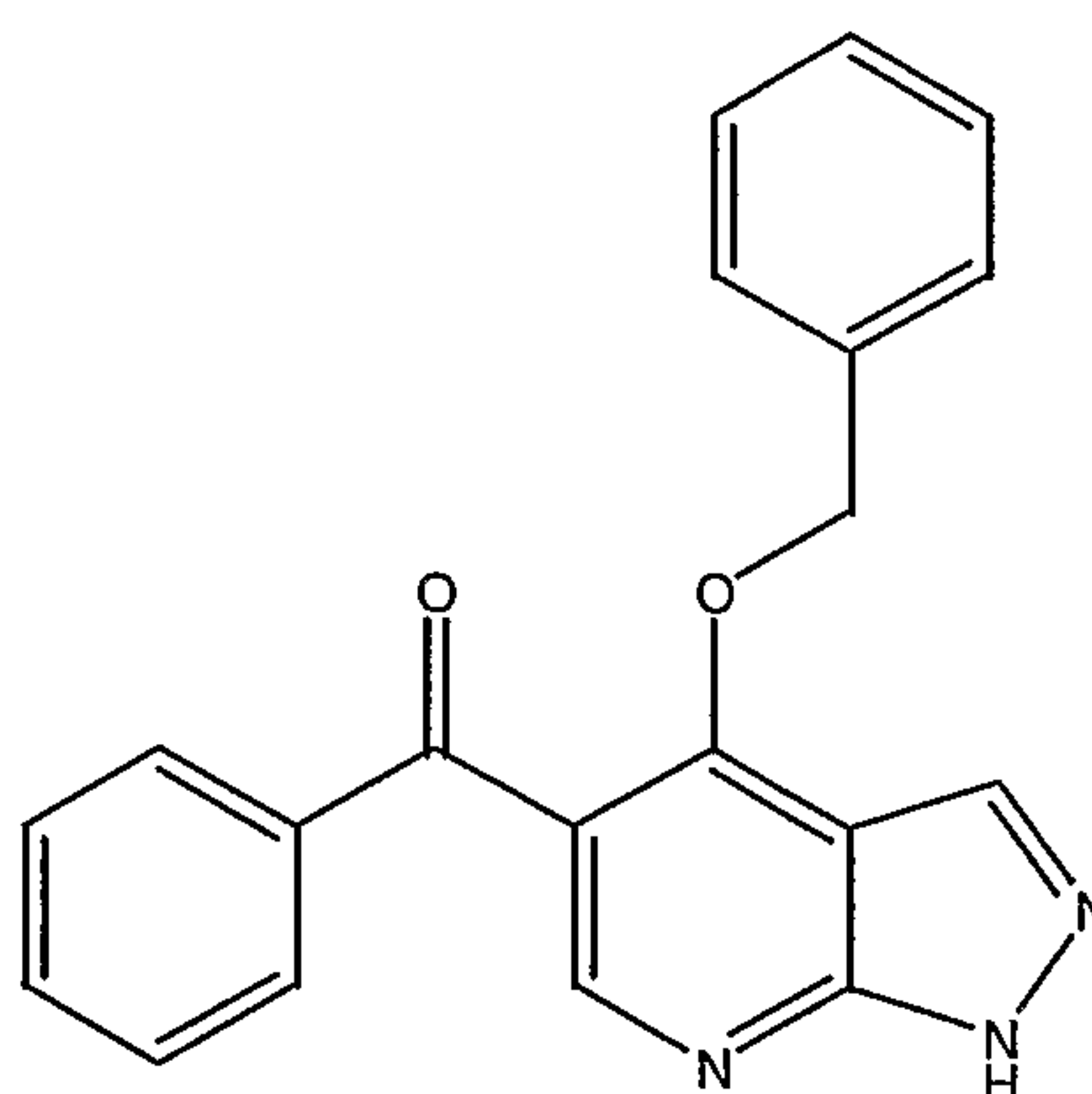
Formula II
