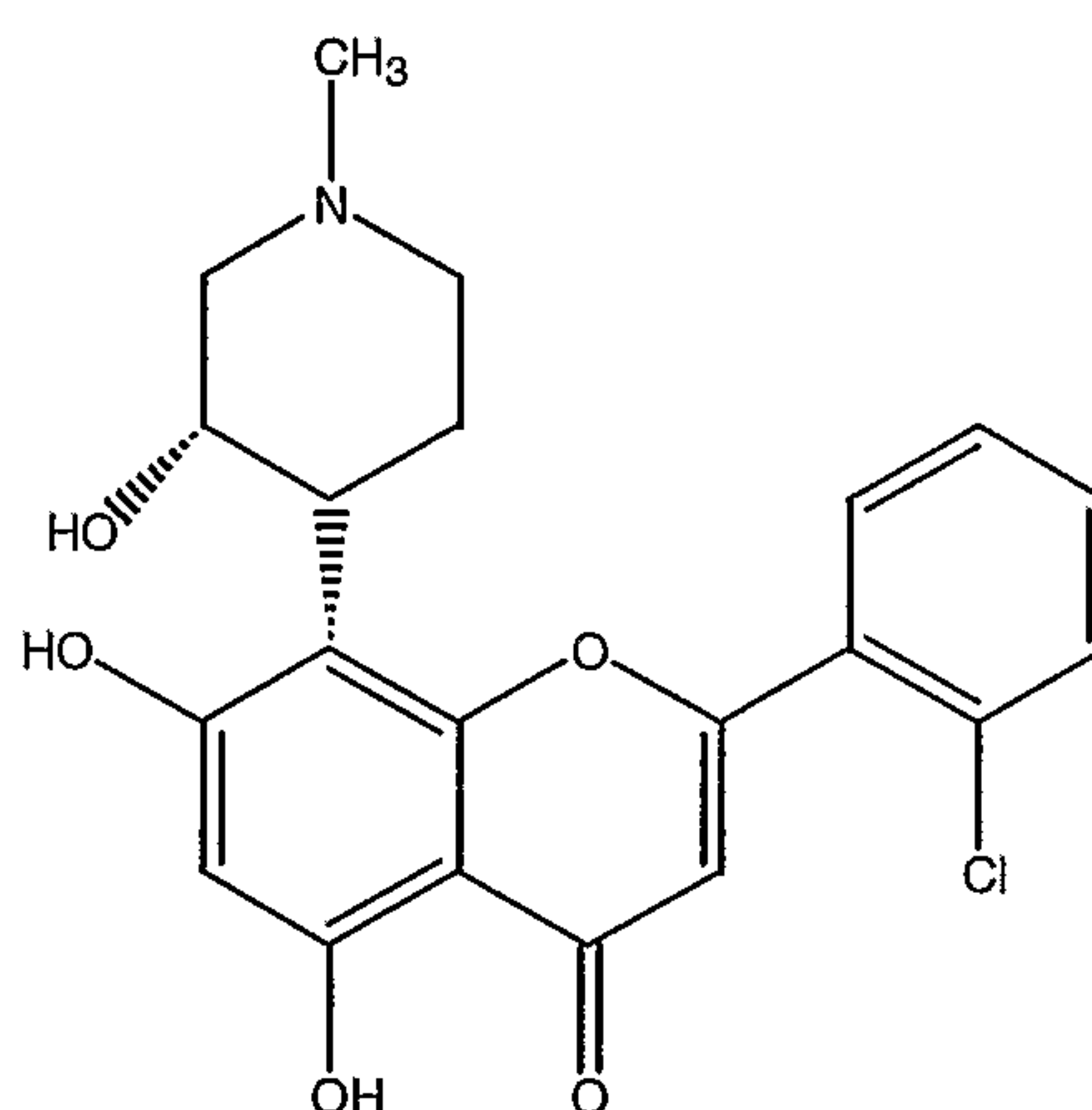
Formula I
