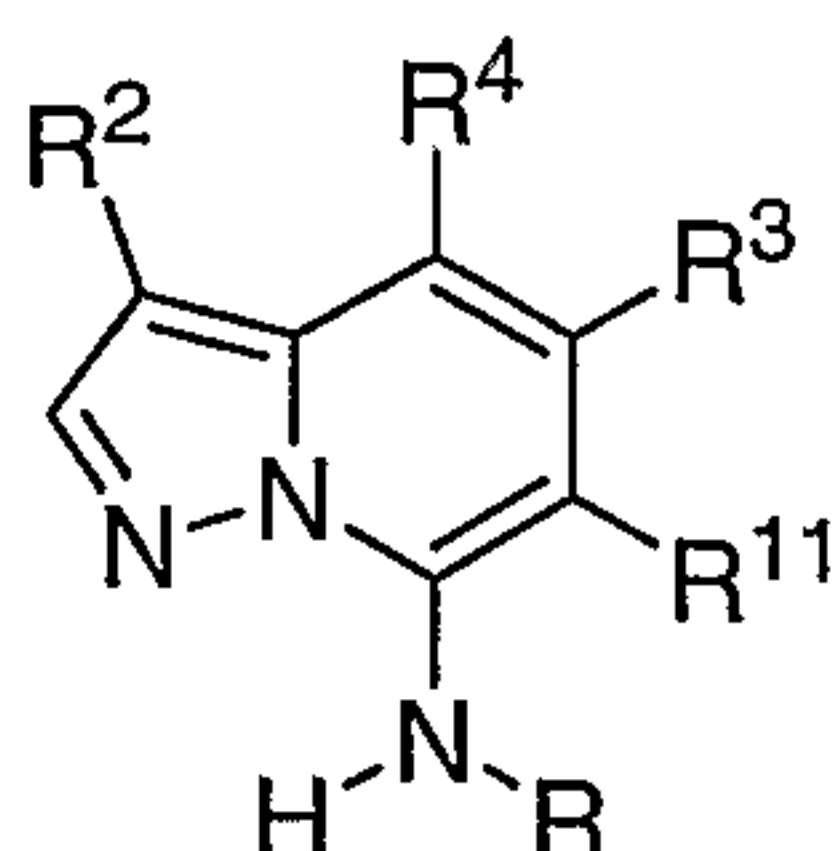
pyrazolopyridine
