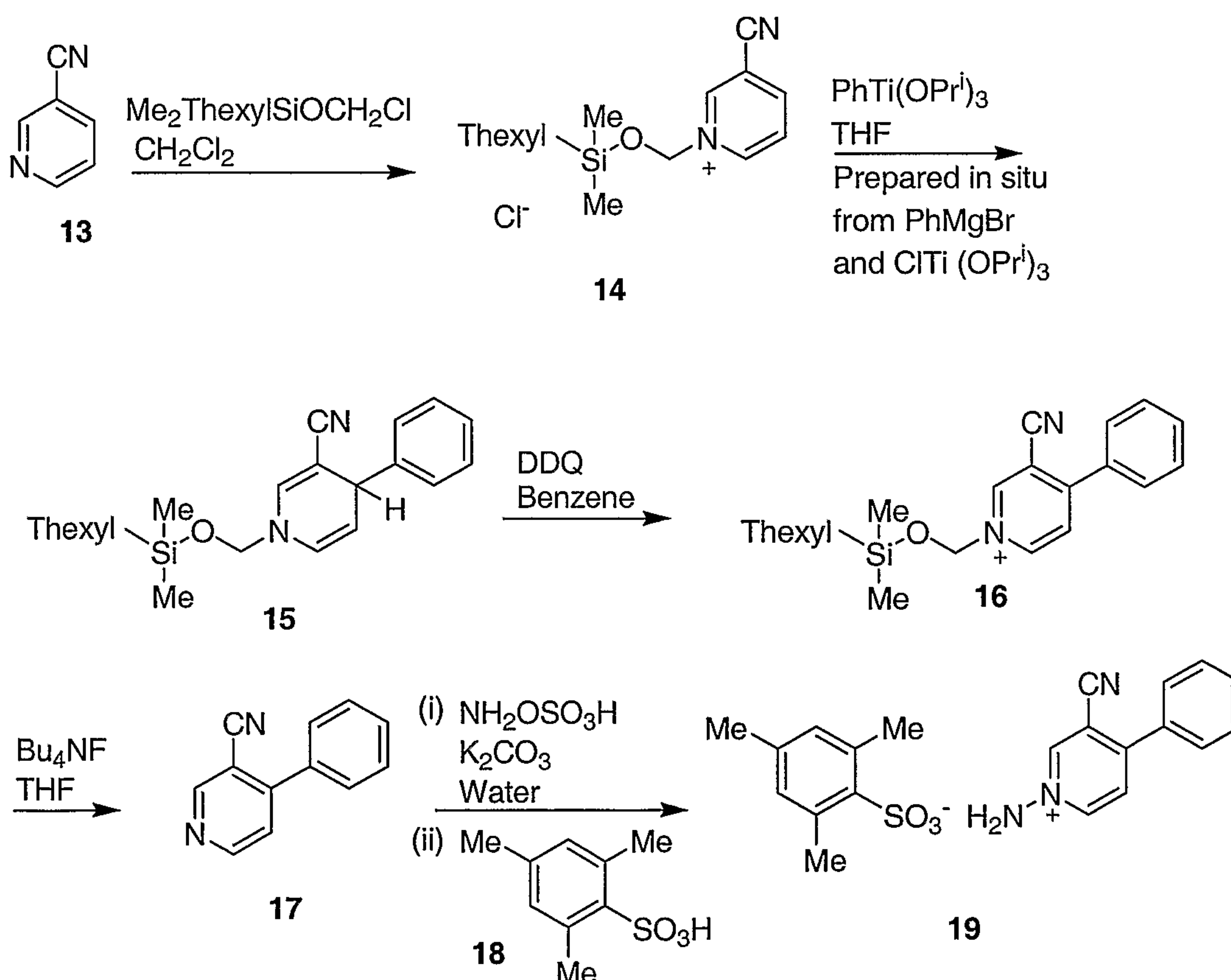
Scheme 1b
