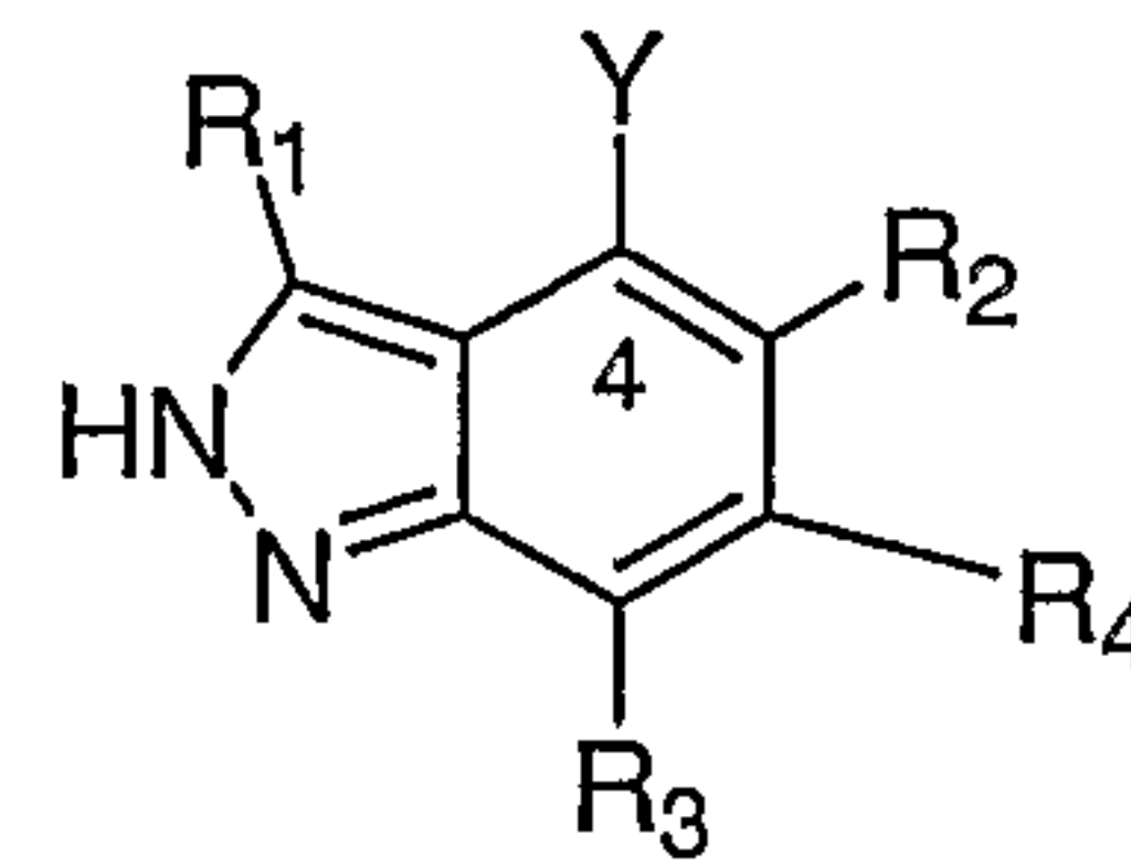
Formula VII
