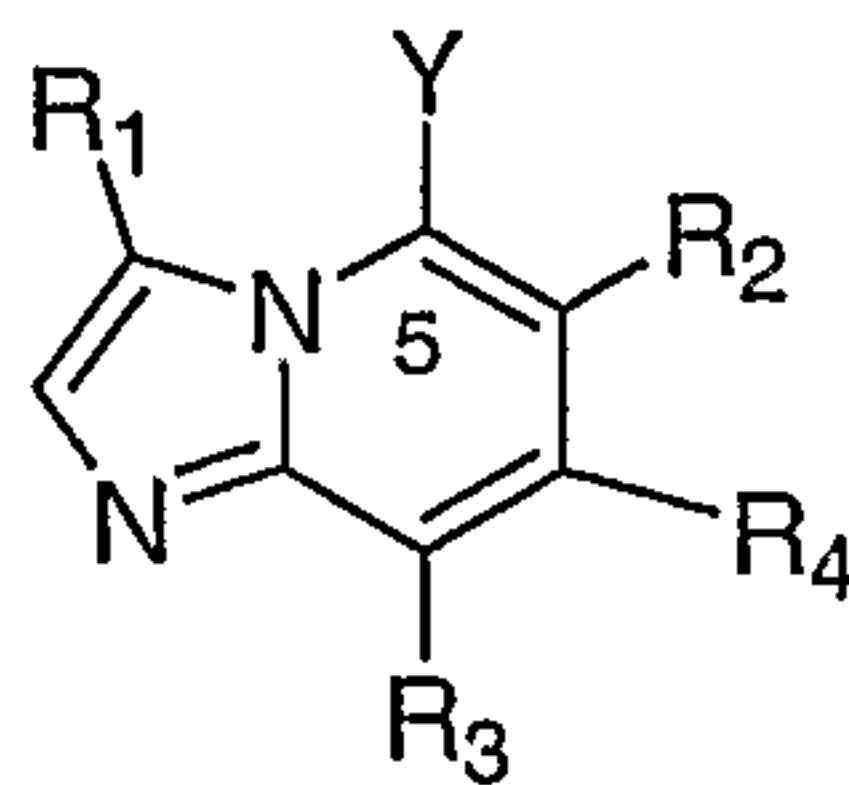
Formula V
