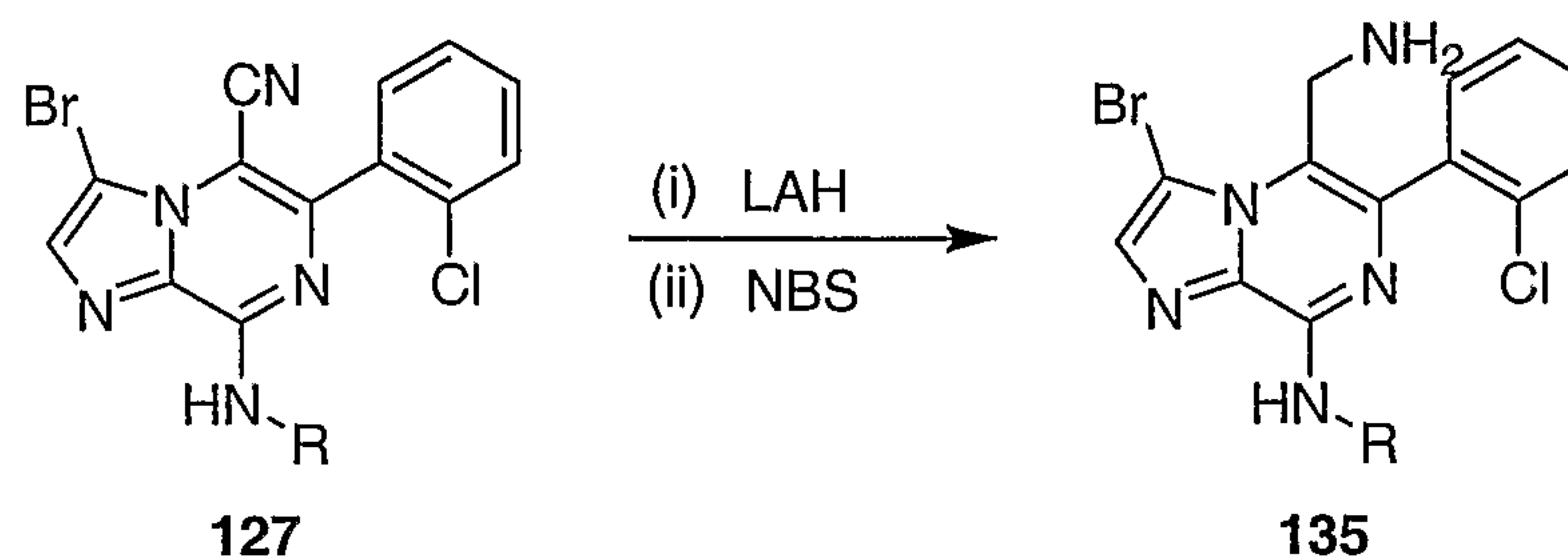
Scheme 3c
