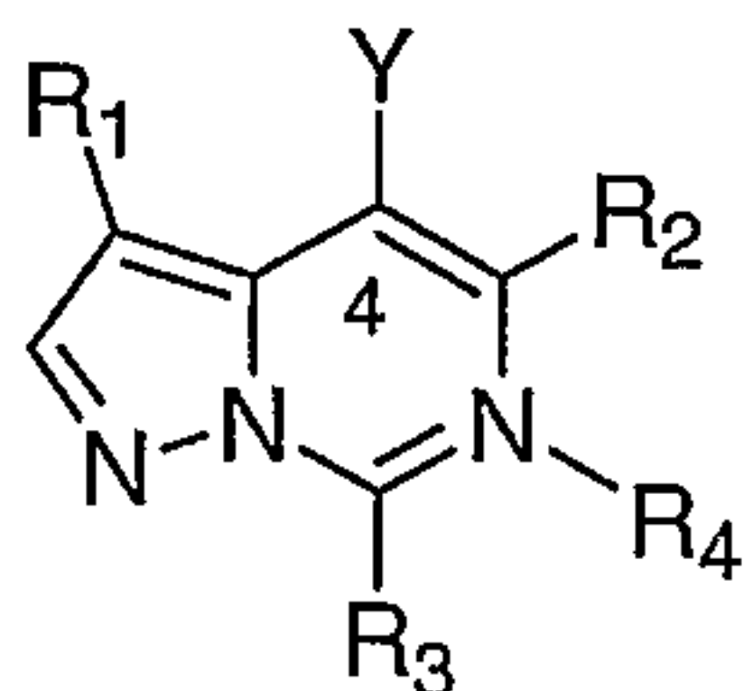
Formula IV
