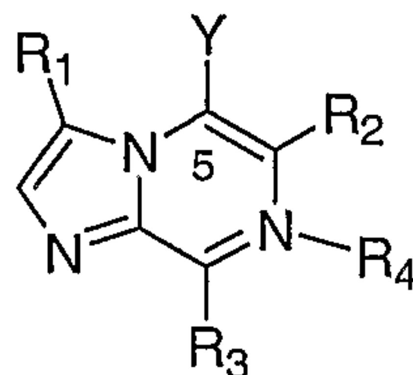
Formula VI
