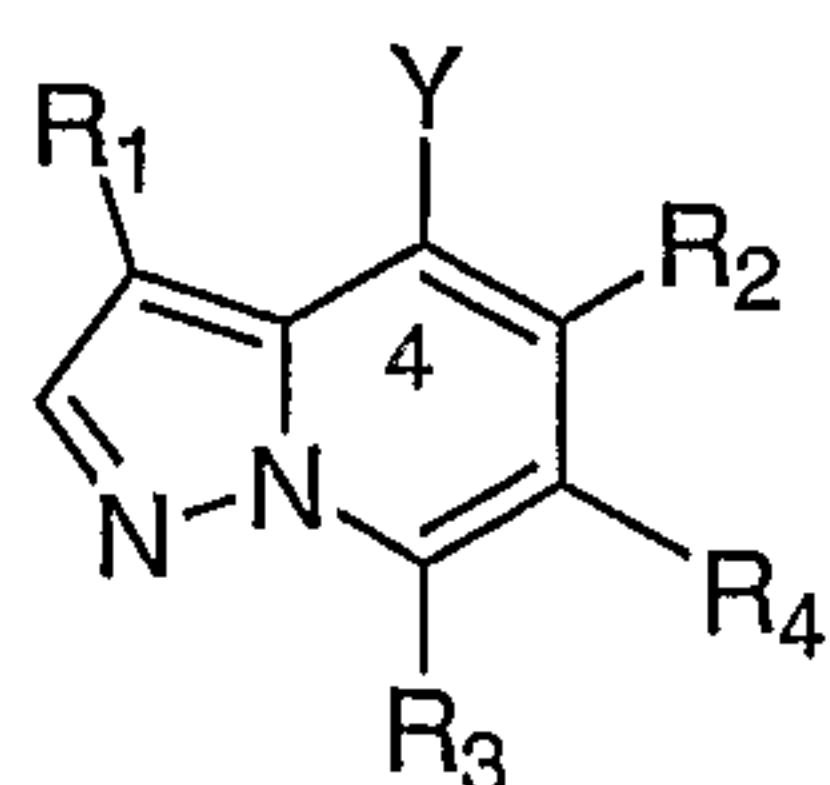
Formula III
