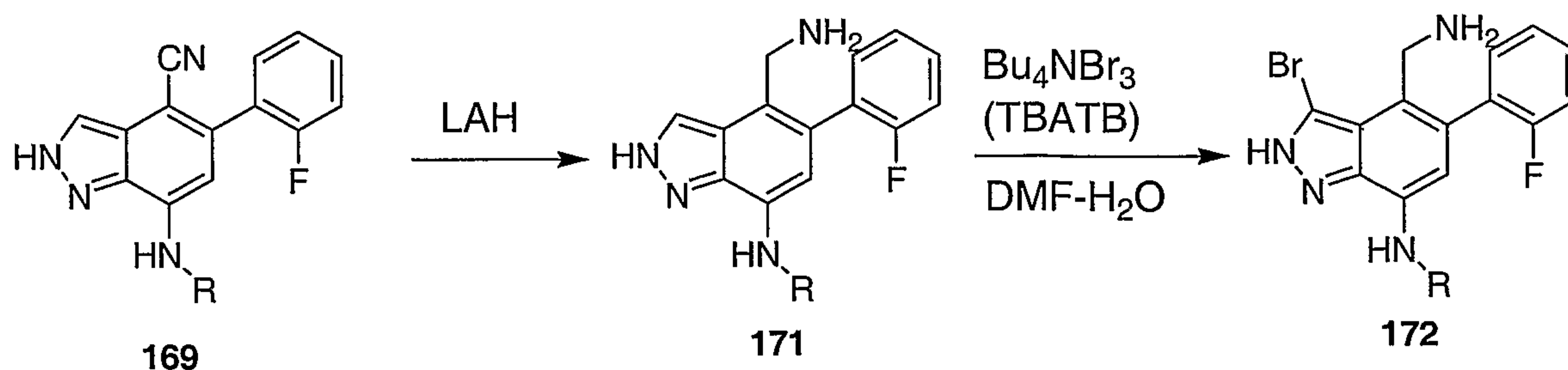
Scheme 5a
