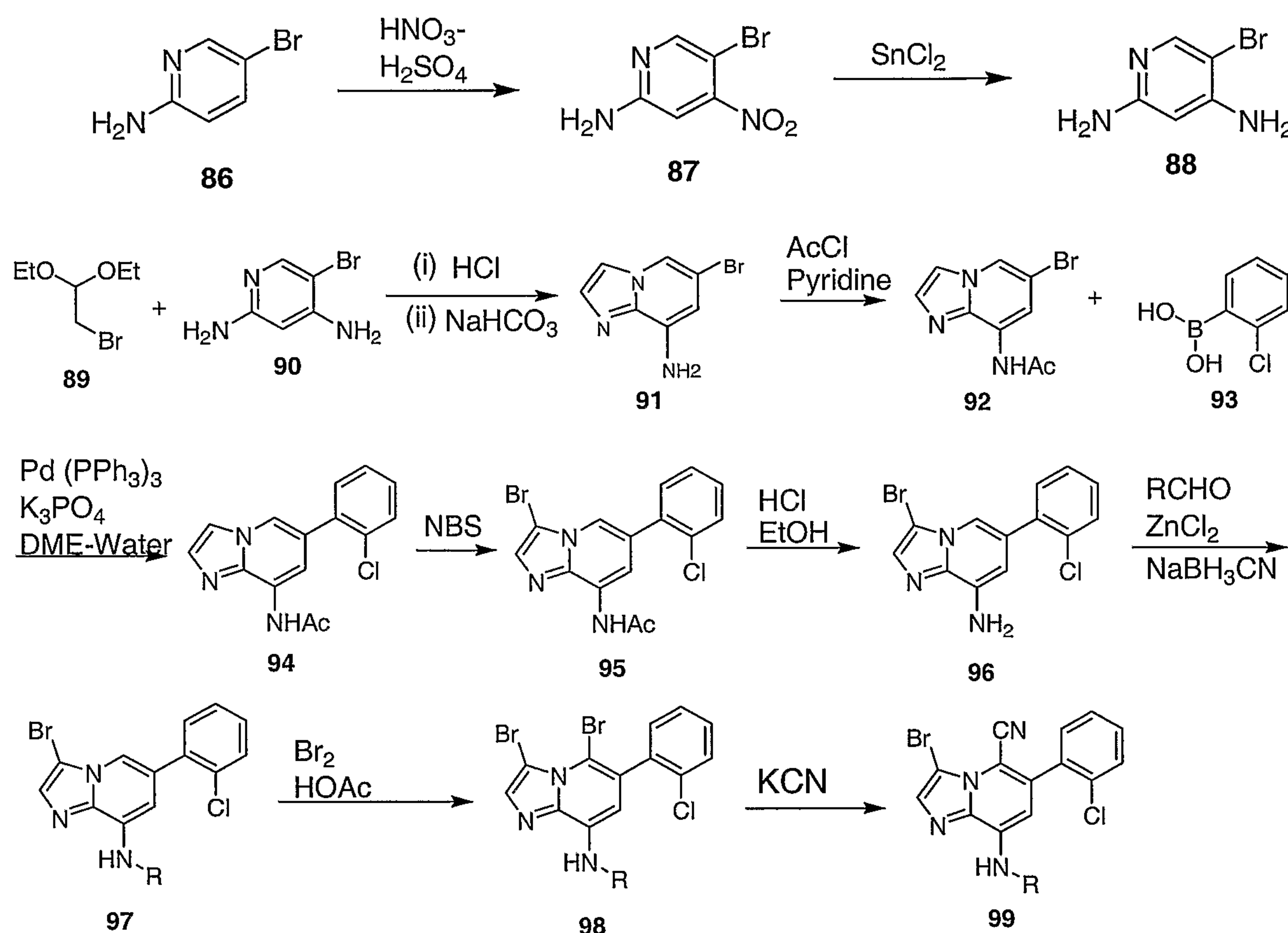
Scheme 2
