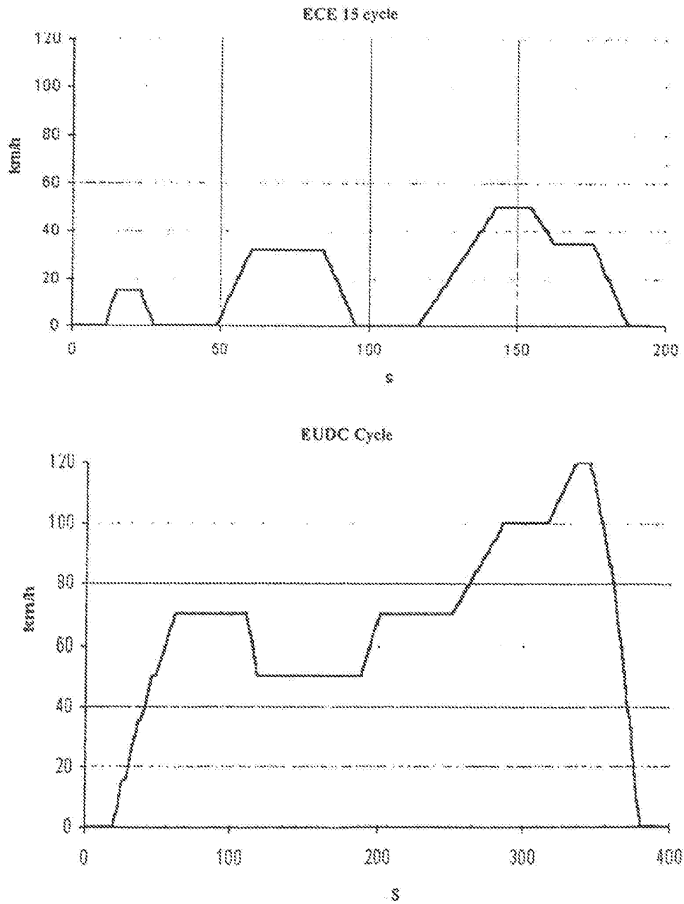
Figure 1 Description of the NEDC cycle
