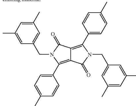
Compound 1
