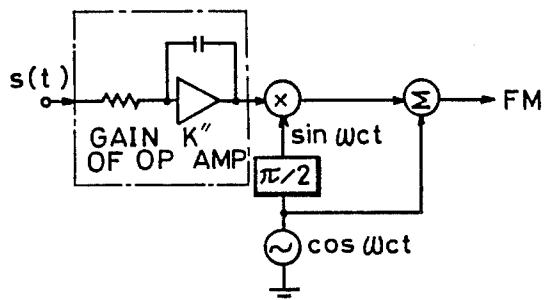
FIG. 4C PRIOR ART
