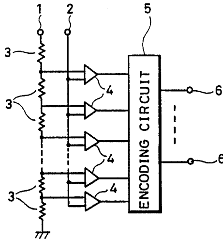
FIG. 6 PRIOR ART
