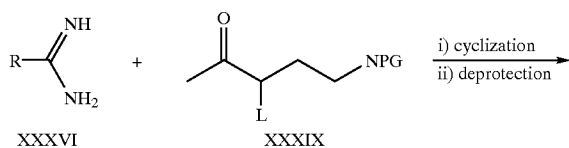
Scheme 16:
