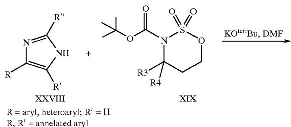
Scheme 12:
