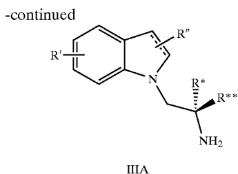
Scheme 8:
