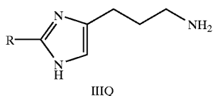
Scheme 17:
