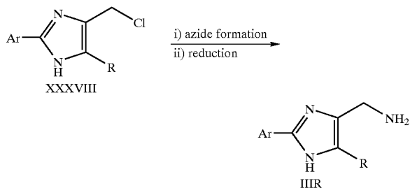
Scheme 15:
