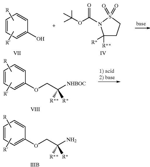
Scheme 18:
