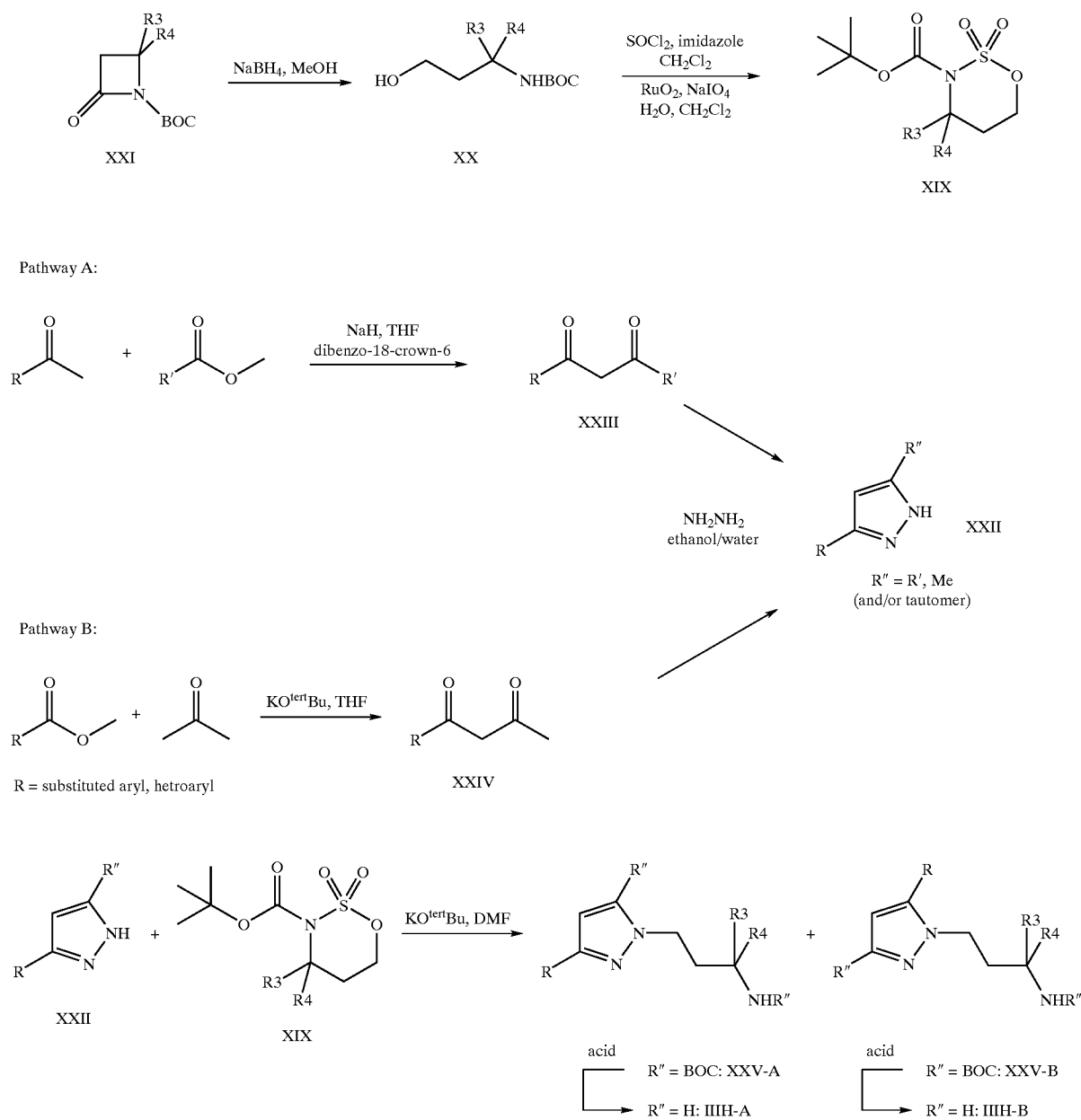
Scheme 10:
