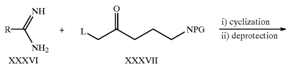
Scheme 14:
