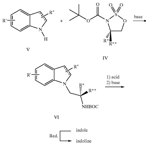
Scheme 6:
