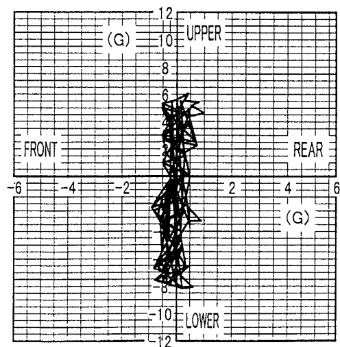
WAVE COMPOSITE OF THE ACCLERATION OF THE ROLL(FOR 0.6 SEC)
