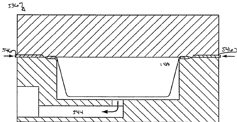
FIG.60
