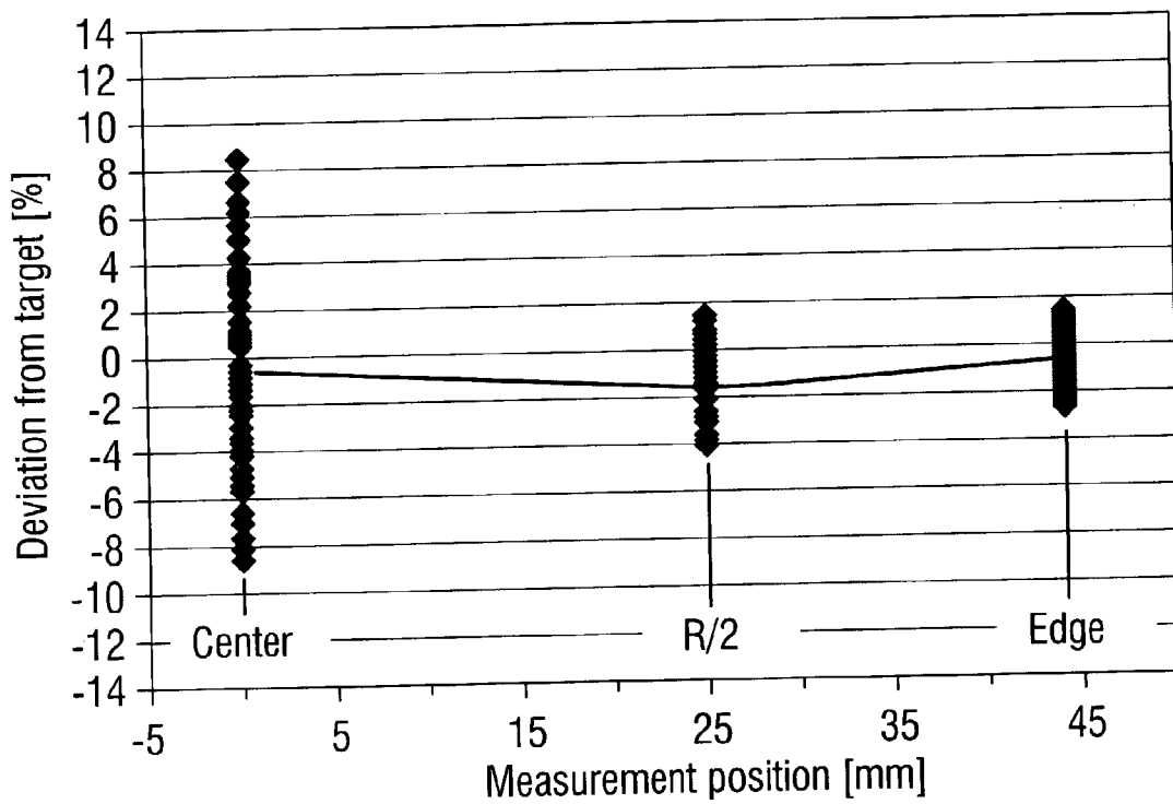
Radial resistance profile for 4" Wafer Float zone pulling process with rotating magnetic field
