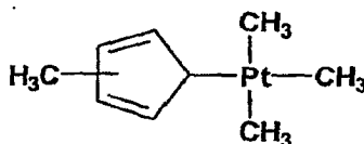
(Trimethyl)methylcyclopentadienylplatinum (IV) ("TMMCP")
