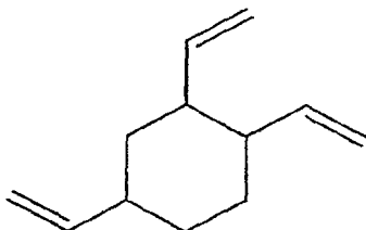
1,2,4-Trivinylcyclohexane CAS # 2855-27-8
