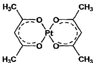
Platinum (II) 2,4-pentanedionate ("Pt(acac) 2 ")
