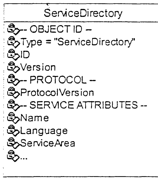
Figure 4: Structure of Service Directory
