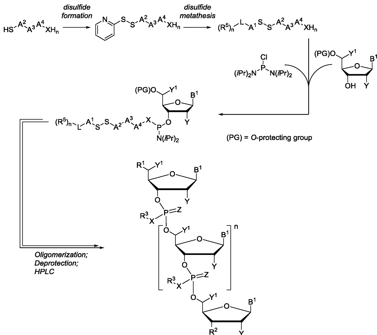
Scheme 1
