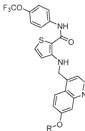
derivatized c-Ki/KDR kinase inhibitor OSI-930
