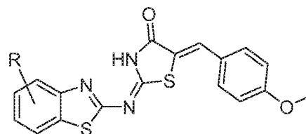
derivatized inhibitor of SHP-2 Domain of Tyrosine Phosphatase
