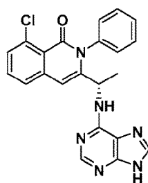
Compound 292
