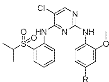
derivatized TAE684
