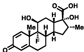
Dex-acid derived from dexamethazone
