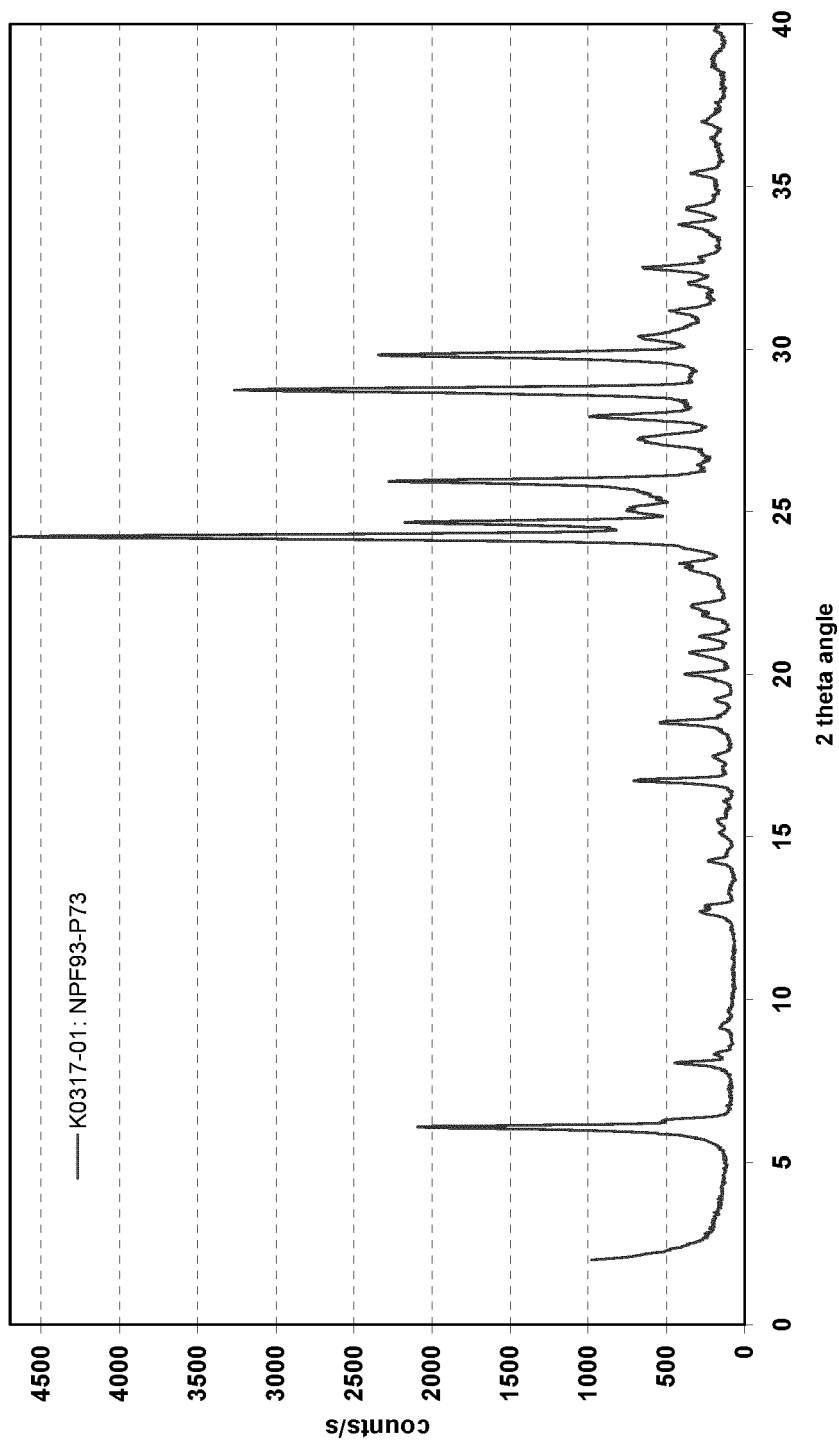
Figure 12 Powder X-ray Diffraction Pattern of (6R)-L-erythro-Tetrahydrobiopterin Dihydrochloride Form I
