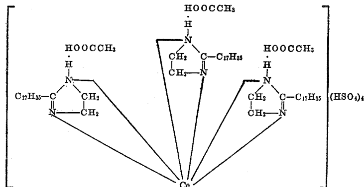
Tri(2-heptadecylimidazoline acetic acid) cerium IV hydrogen sulfate, C_{66}H_{136}O_{22}N_6S_4Ce
