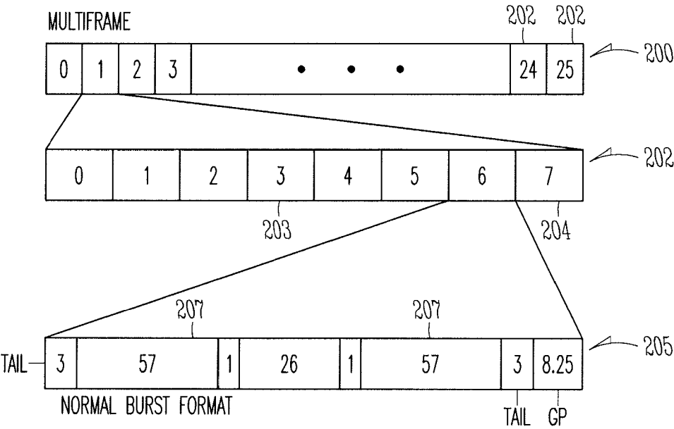
FRAME STRUCTURE
