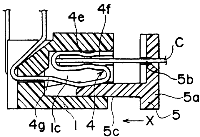
Fig. 10 Prior Art
