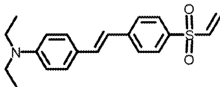
5 {4-[2-(4-Ethenesulfonyl-phenyl)-vinyl]-phenyl}-diethyl-amine
