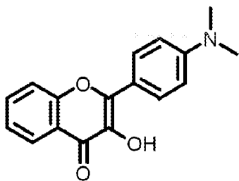
3-hydroxy-4'-N,N-dimethylaminoflavone
