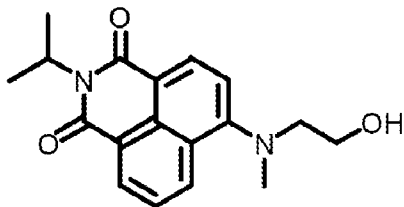
(2-hydroxyethyl)(methyl)amino)-2-isopropyl-1H-benzo[de]isoquinoline-1,3(2H)-dione
