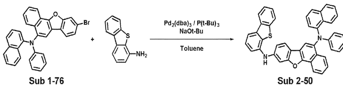
Reaction Scheme 19
