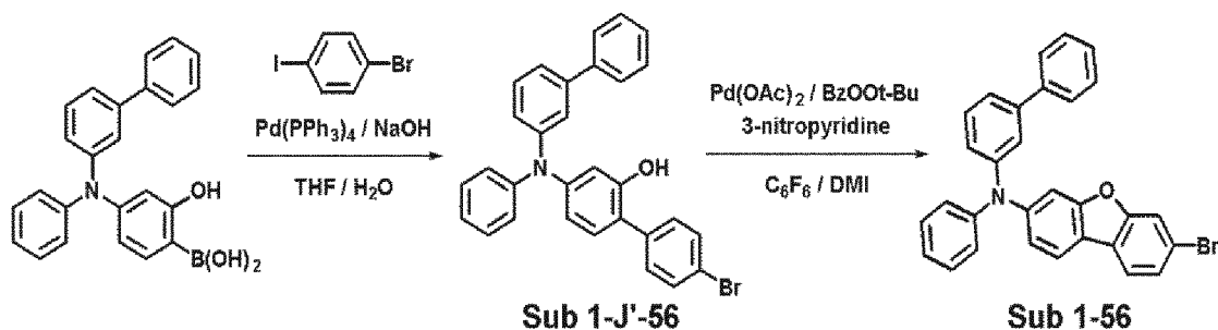
Reaction Scheme 7
