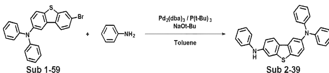
Reaction Scheme 18
