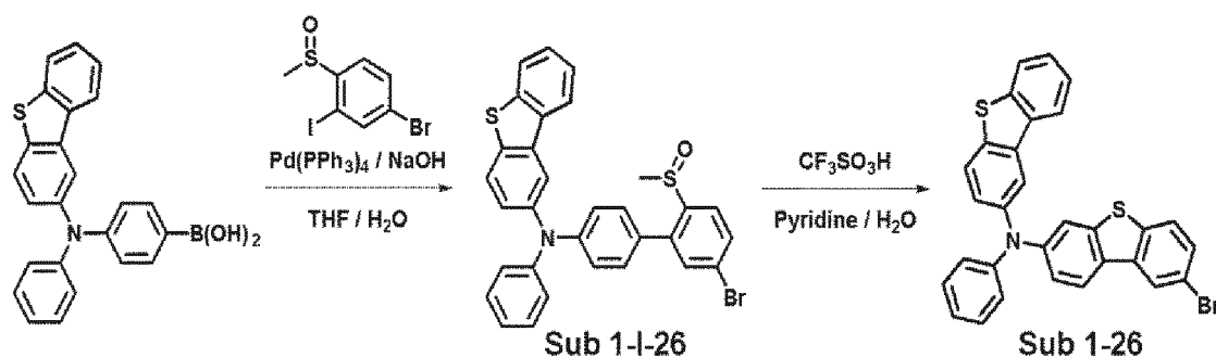
Reaction Scheme 6
