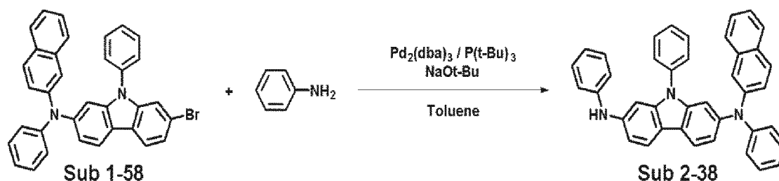
Reaction Scheme 17
