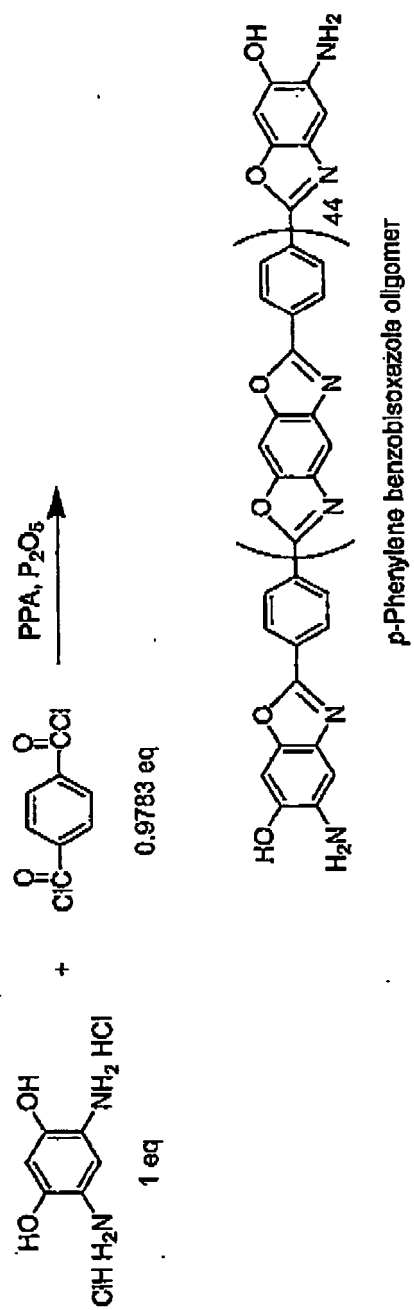
Scheme 5
