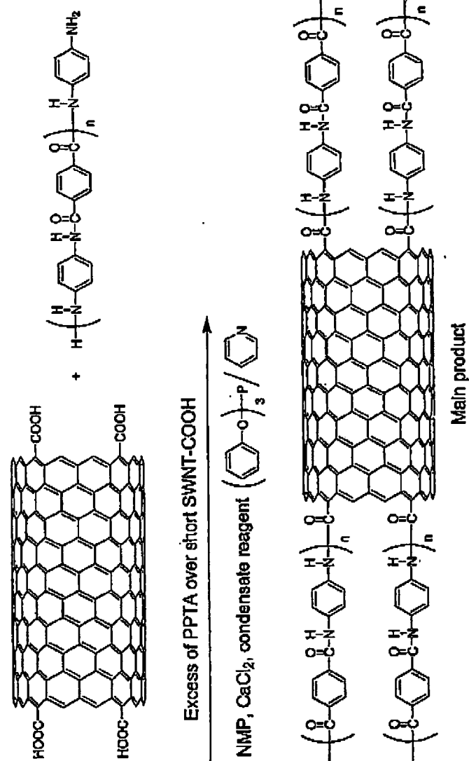
Scheme 12
