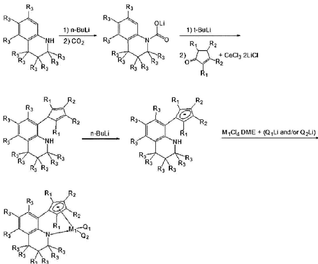
[Reaction Scheme 1]
