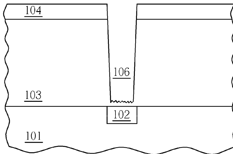
FIG. 4 PRIOR ART
