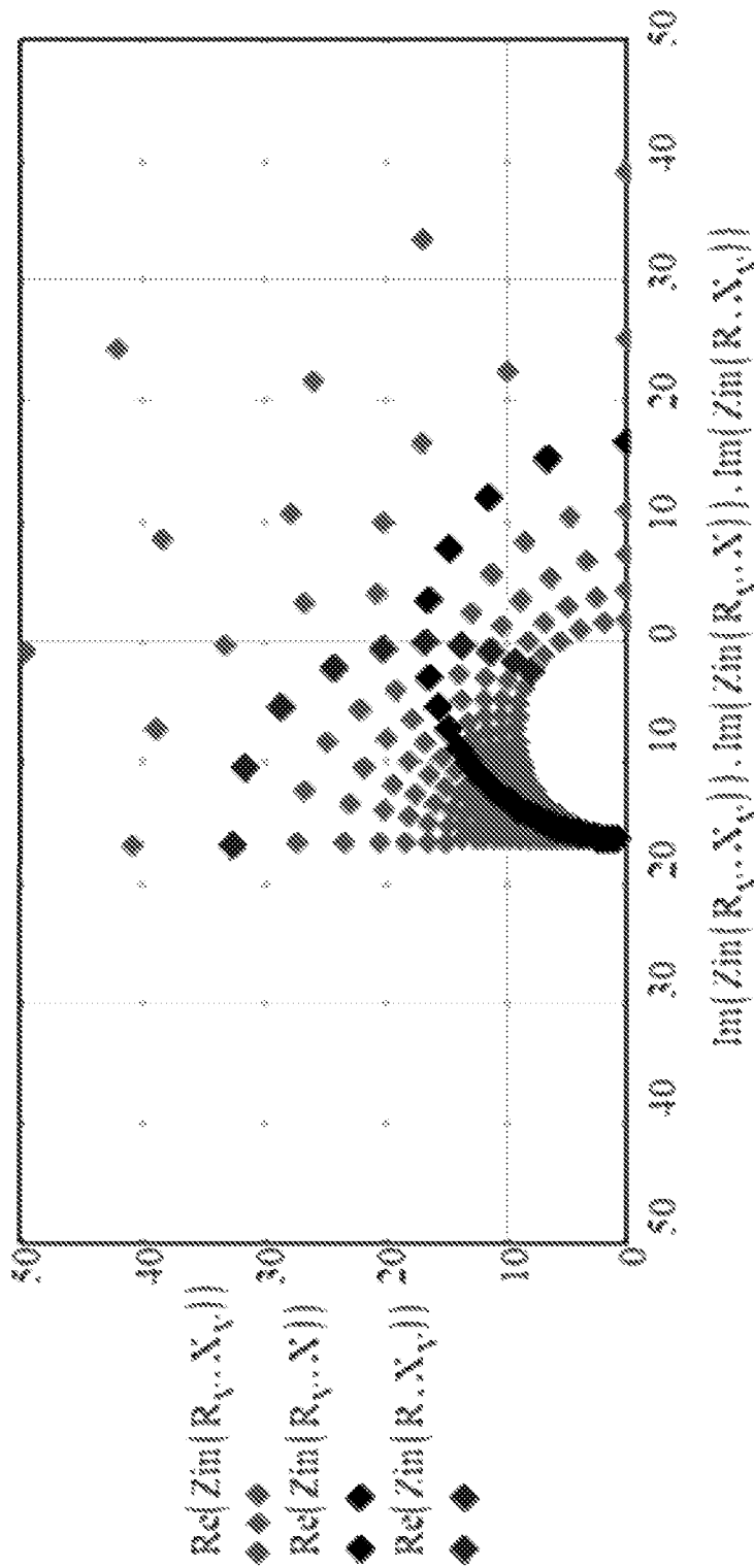
Z_{in}(\text{XFRM}) versus a wide range in R_{in}(\text{Tx})
