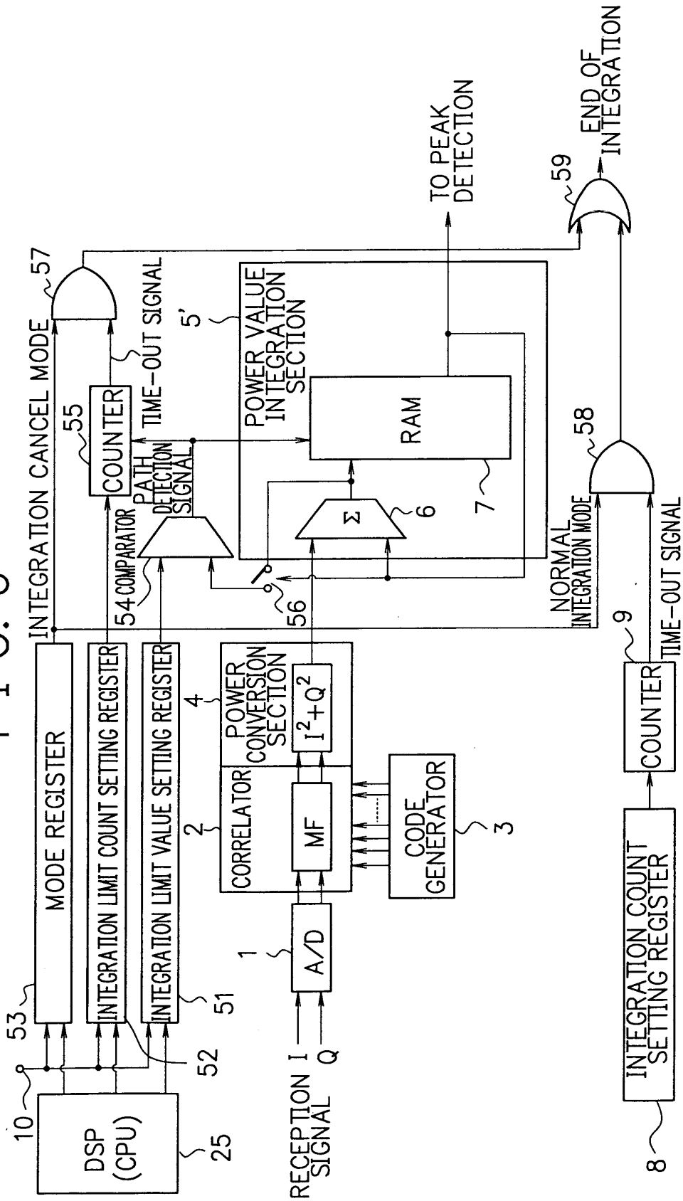
BLOCK DIAGRAM OF CELL SEARCH OF SECOND EMBODIMENT
