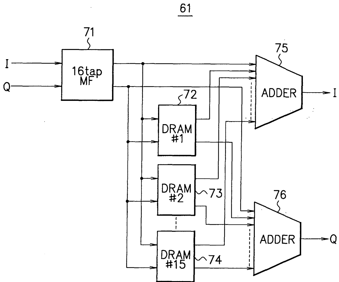
BLOCK DIAGRAM OF CORRELATOR OF THIRD EMBODIMENT
