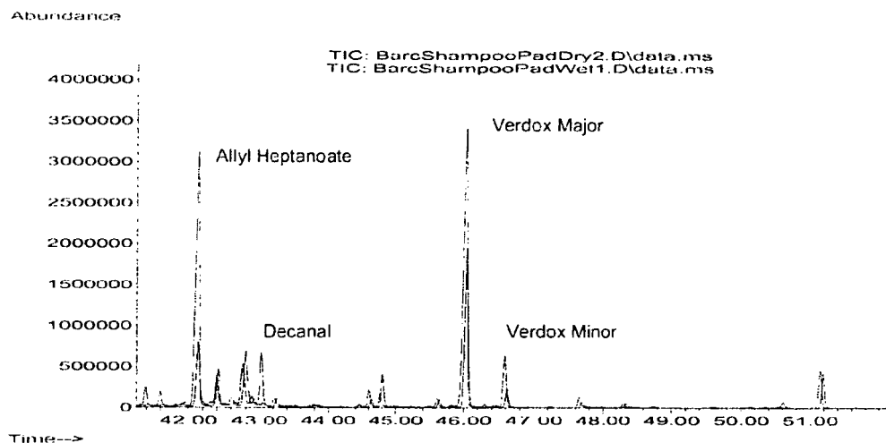
Figure 8. GC/MS Headspace ratio of perfume raw materials (PRM) from the dissolved shampoo pad vs. the neat liquid shampoo control
