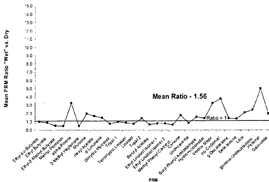
Figure 5. GC/MS Headspace ratio of perfume raw materials (PRM) from the dissolved shampoo pad (7:1 water dilution) vs. the original dry shampoo pad
