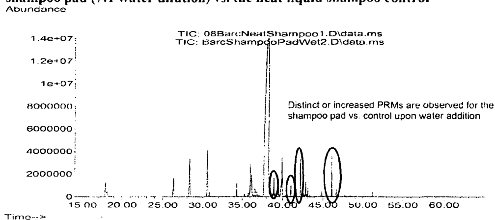
Figure 10. GC headspace abundance of perfume raw materials from the dissolved shampoo pad (7:1 water dilution) vs. the neat liquid shampoo control
