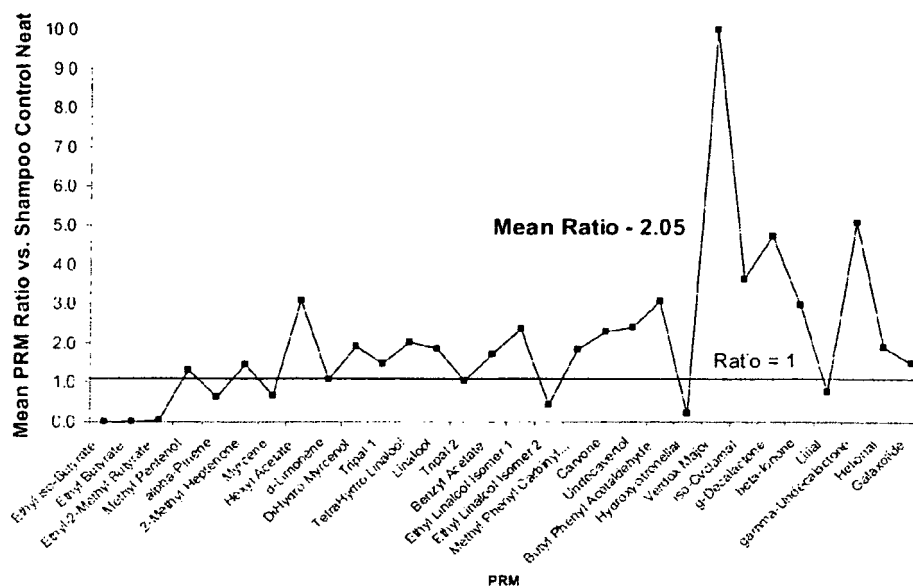
Figure 8. GC/MS Headspace ratio of perfume raw materials (PRM) from the dissolved shampoo pad vs. the neat liquid shampoo control
