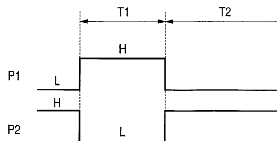
(Prior Art) FIG. 7
