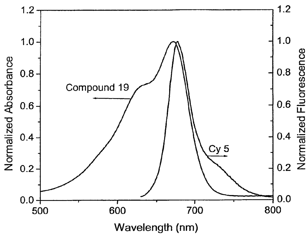
FIG. 10. Spectral overlap of compound 19 with Cy5.
