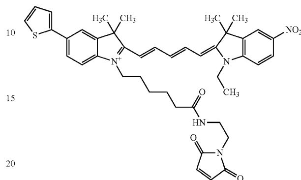
Example 28
