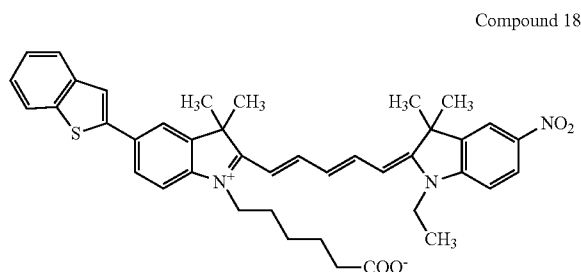
Compound 18
