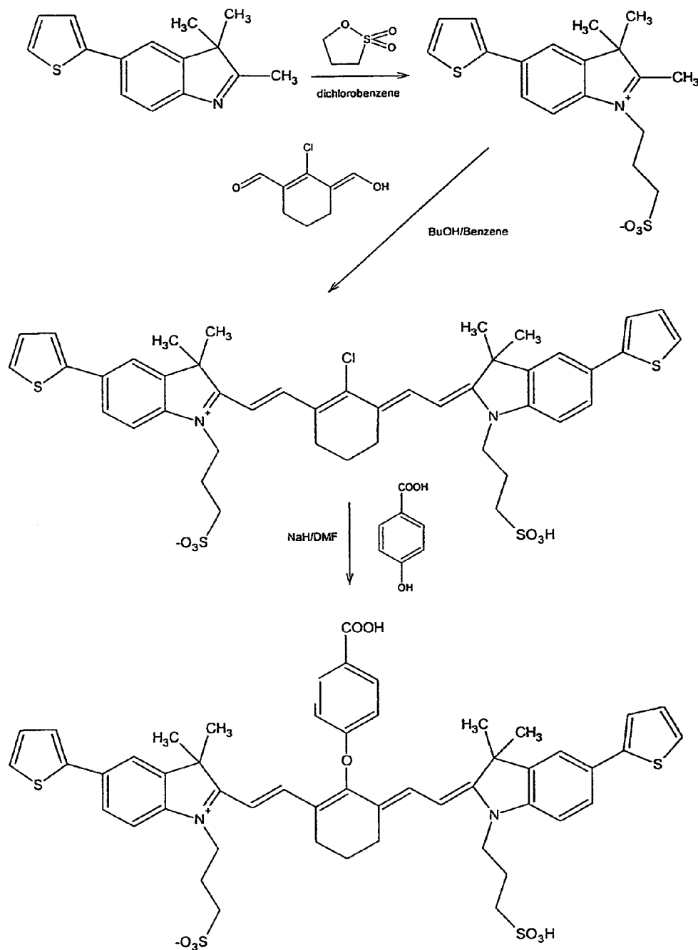
FIG. 3. Synthesis of a cyanine that has a RM at the BRIDGE atoms
