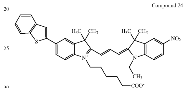
Compound 24
