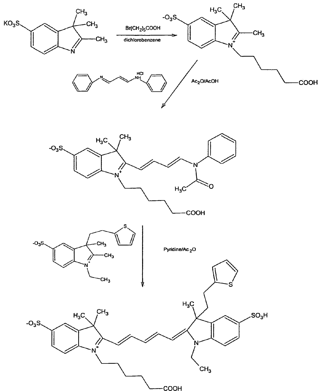
FIG. 5. Synthesis of a cyanine that has a LQM at 3-position
