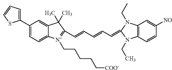
Compound 19
