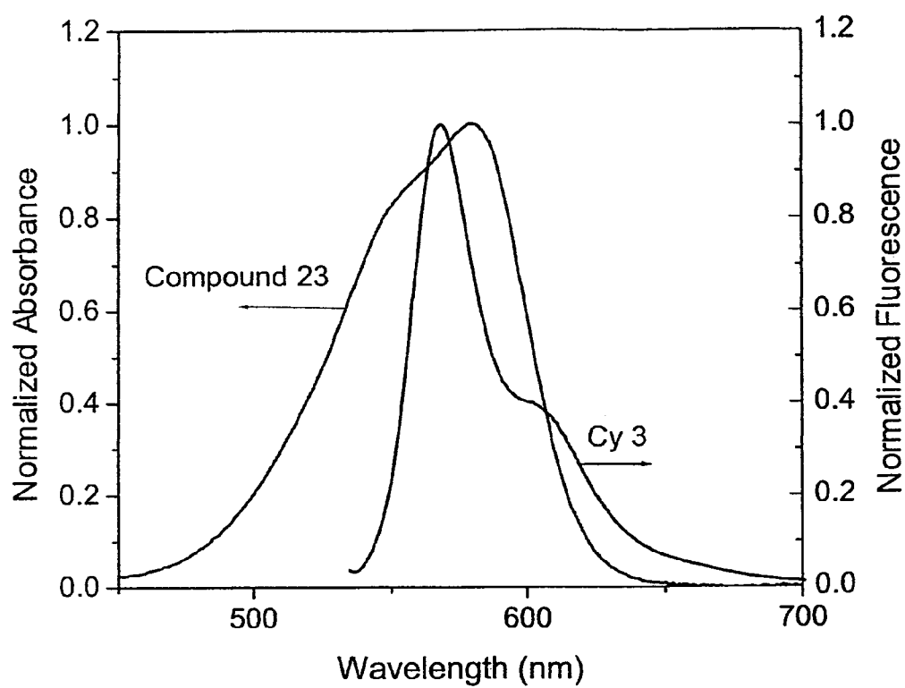
FIG. 9. Spectral overlap of compound 23 with Cy3
