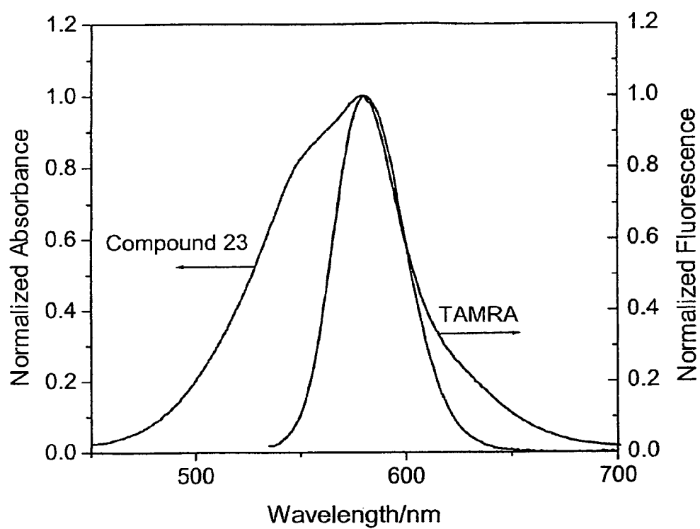
FIG. 8. Spectral overlap of compound 23 with 5-TAMRA
