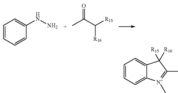
Scheme 1. Typical synthesis of indolium intermediates
