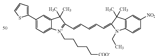
Compound 16
