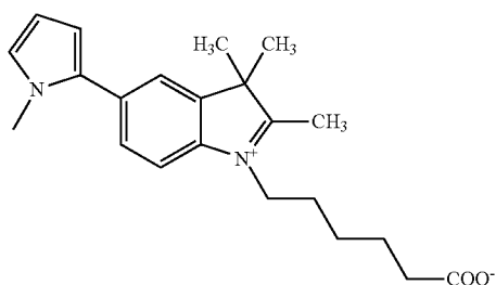
Compound 21
