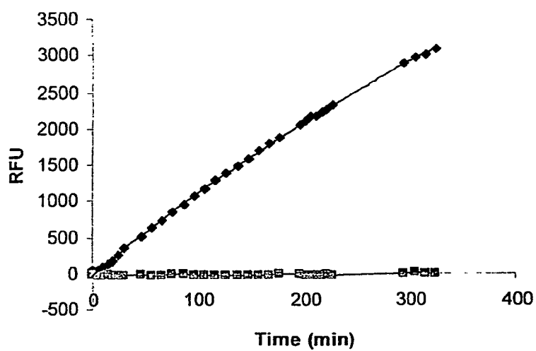
FIG. 11. MMP-2 cleavage of Compound 19-Lys-Pro-Leu-Ala-Nva-Asp(Cy5)-Ala-Arg-NH 2 .
