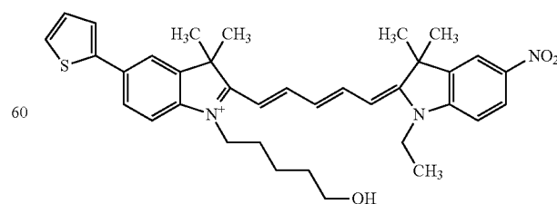
Compound 30
