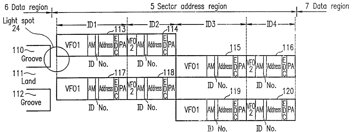
Data arrangement in address blocks
