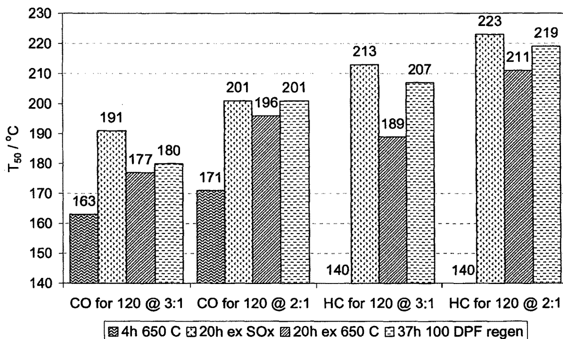
Figure 17: Impact of Pt:Pd ratio on performance of conventional DOC, 120 gcF PGM at 3:1 versus 2:1 Pt:Pd.
