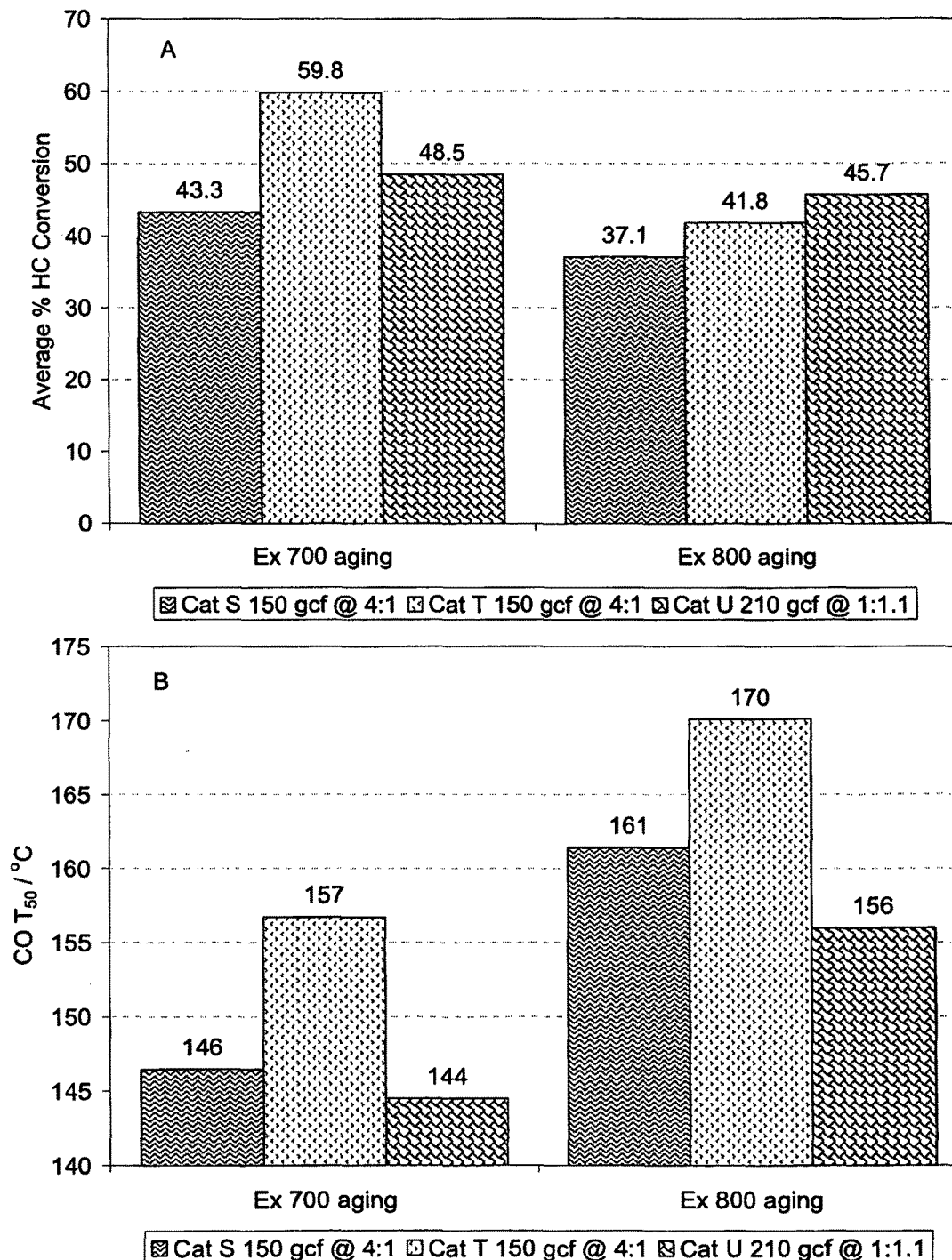
Figure 15: SGB testing/oven aging of conventional DOCs, 150 gcf PGM at 4:1 vs 'Quench resistant high Pd DOC, 210 gcf PGM @ 1:1.1 using complex HC mix.
