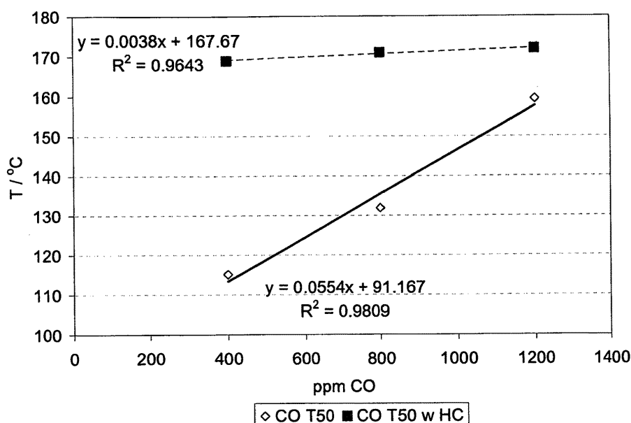
Figure 1: Impact of Propene/Propane on CO light-off ( T_{50} ) for conventional PtPd DOC 120 gcf @ 3:1 in SGB test. (1*3" core, aged at 650C 10% steam/air for 20h)
