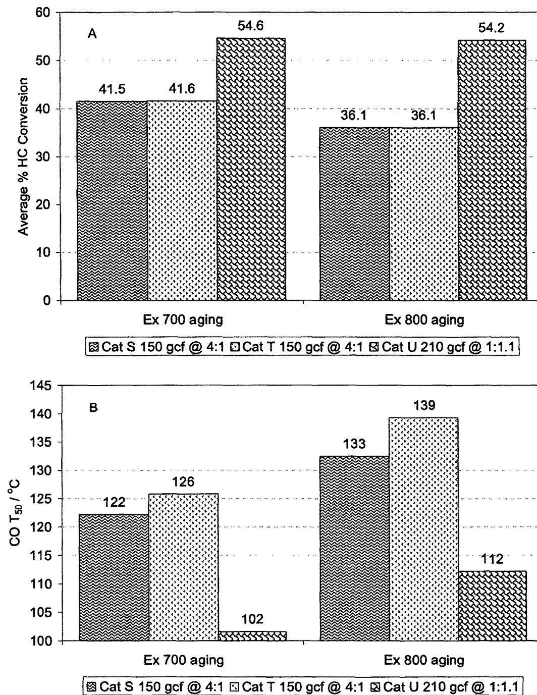
Figure 16: SGB testing/oven aging of conventional DOCs, 150 PGM at 4:1 vs 'Quench' resistant high Pd DOC, 210 gcf PGM @ 1:1.1 using C 3 only HC mix.
