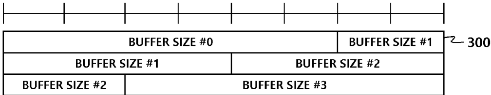
LONG BSR MAC CONTROL ELEMENT FORMAT
